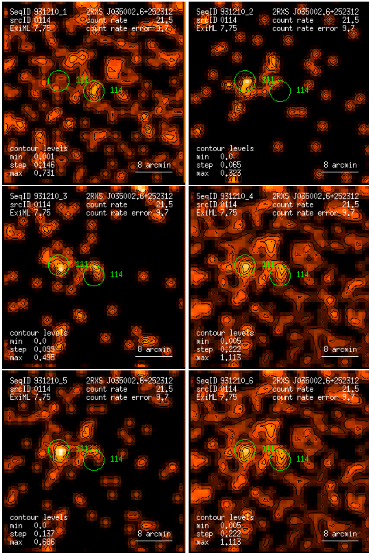
Figure 114: RASS 931210: detection 0114: band rate images, Gaussian filter: (1) PSPC channels 11 – 41, (2) 52 – 90, (3) 91 – 201, (4) 11 – 235, (5) 52 – 201, (6) 11 – 201. Broad band rates in counts/ks. Band rate contour levels in counts/ks/arcmin 2 .
