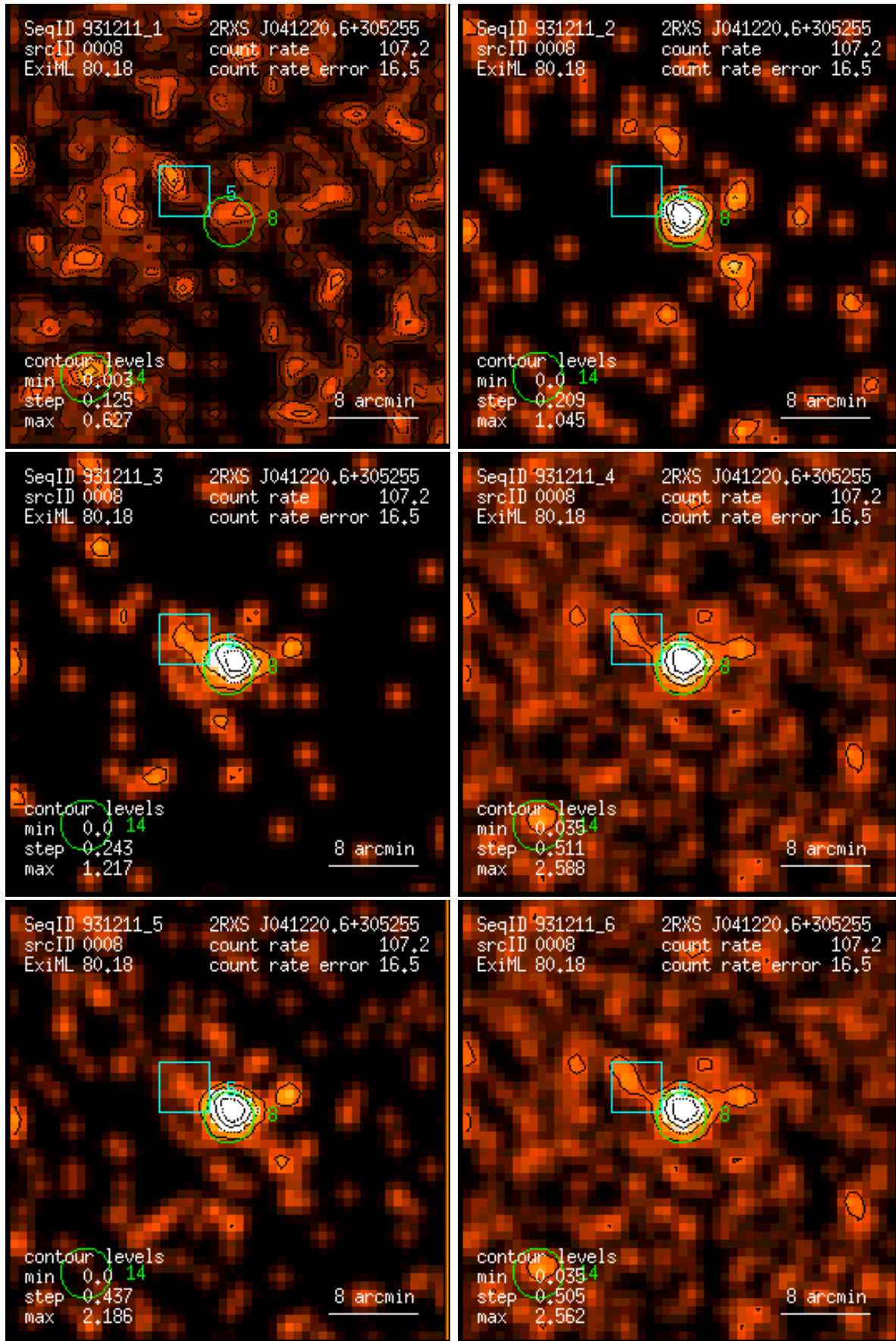
Figure 8: RASS 931211: detection 0008: band rate images, Gaussian filter: (1) PSPC channels 11 – 41, (2) 52 – 90, (3) 91 – 201, (4) 11 – 235, (5) 52 – 201, (6) 11 – 201. Broad band rates in counts/ks. Band rate contour levels in counts/ks/arcmin 2 .
