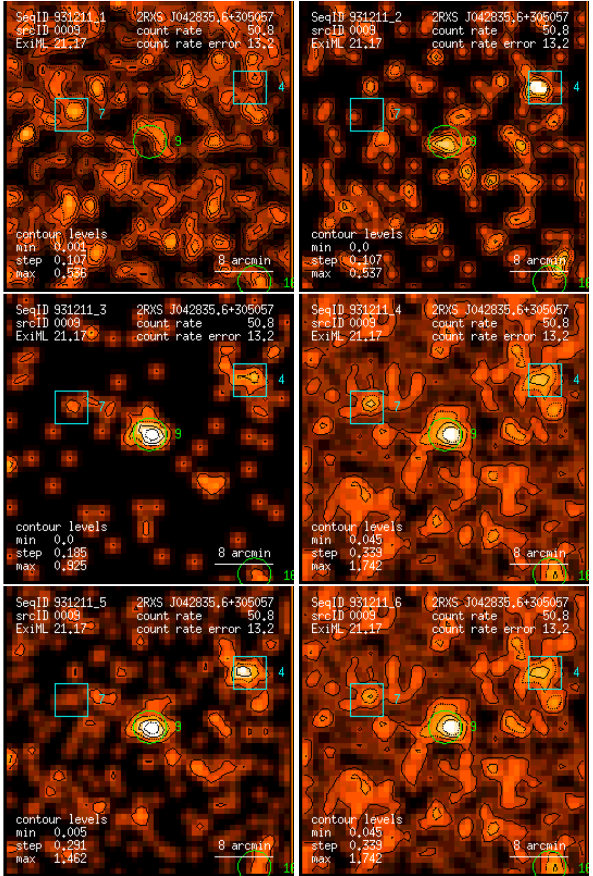
Figure 9: RASS 931211: detection 0009: band rate images, Gaussian filter: (1) PSPC channels 11 – 41, (2) 52 – 90, (3) 91 – 201, (4) 11 – 235, (5) 52 – 201, (6) 11 – 201. Broad band rates in counts/ks. Band rate contour levels in counts/ks/arcmin 2 .
