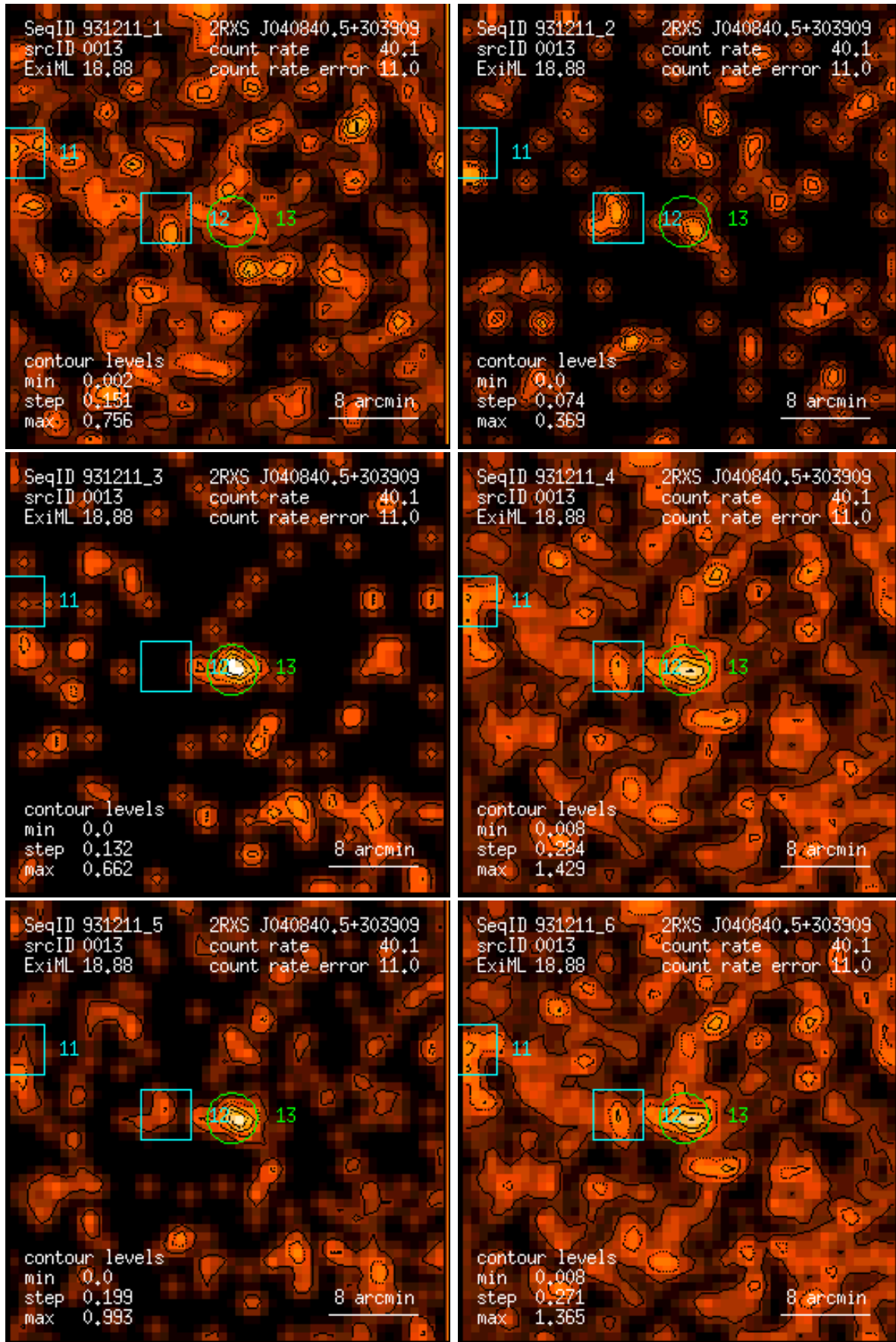
Figure 13: RASS 931211: detection 0013: band rate images, Gaussian filter: (1) PSPC channels 11 – 41, (2) 52 – 90, (3) 91 – 201, (4) 11 – 235, (5) 52 – 201, (6) 11 – 201. Broad band rates in counts/ks. Band rate contour levels in counts/ks/arcmin 2 .
