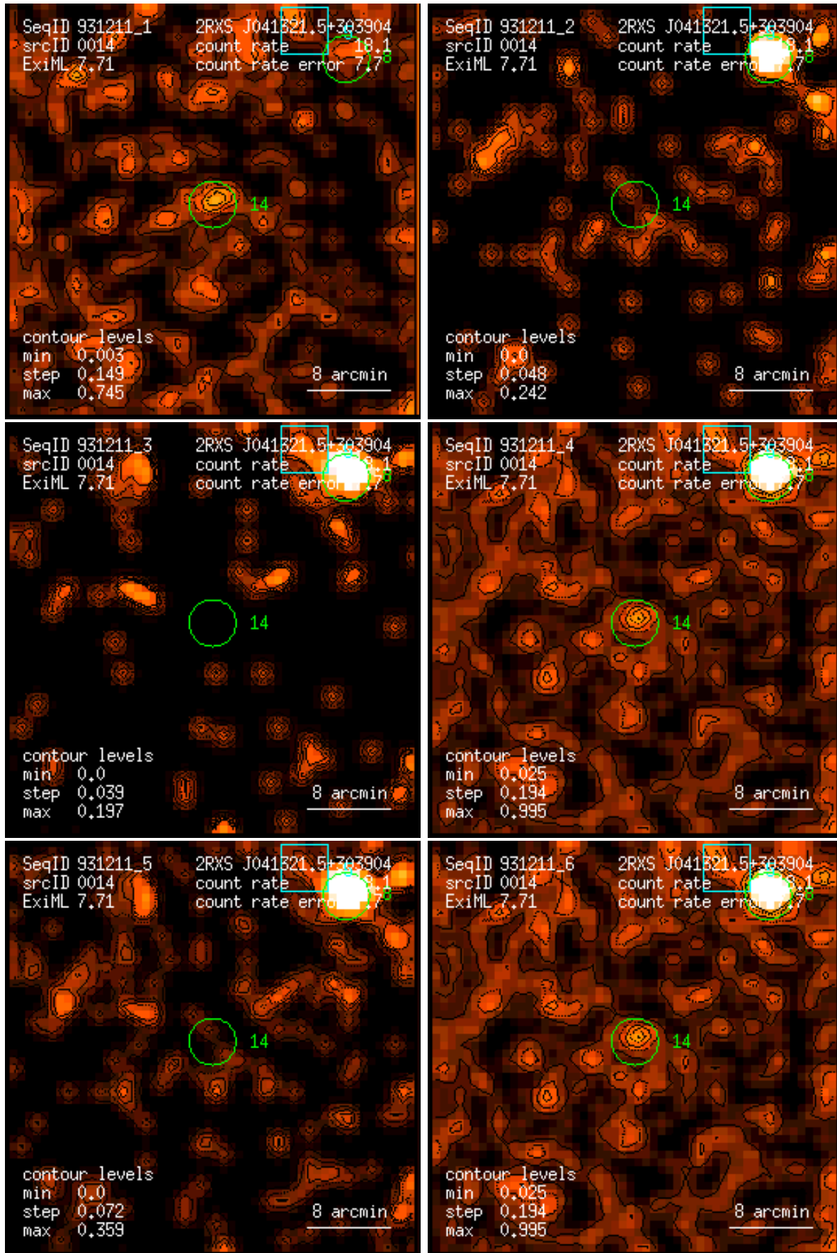
Figure 14: RASS 931211: detection 0014: band rate images, Gaussian filter: (1) PSPC channels 11 – 41, (2) 52 – 90, (3) 91 – 201, (4) 11 – 235, (5) 52 – 201, (6) 11 – 201. Broad band rates in counts/ks. Band rate contour levels in counts/ks/arcmin 2 .
