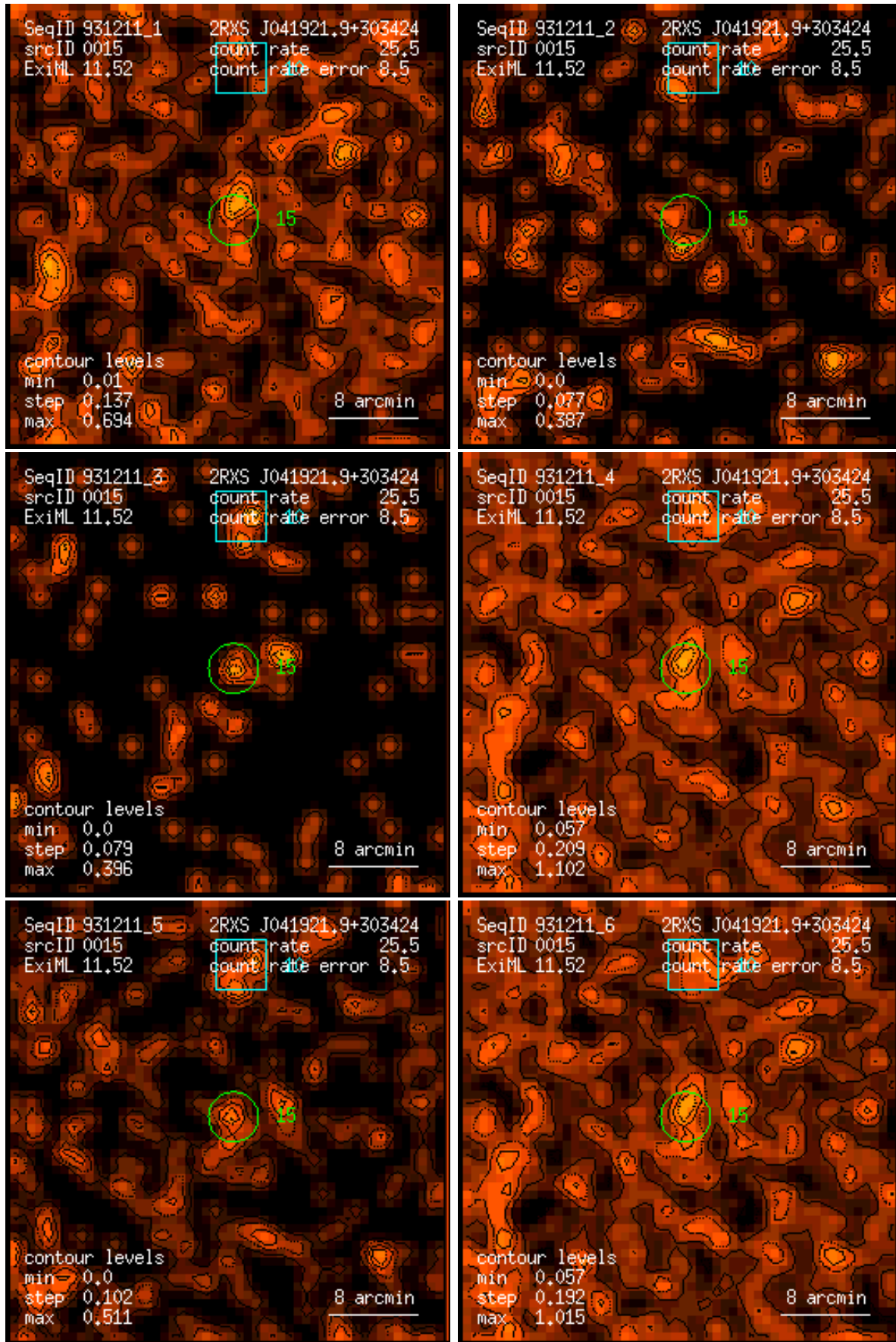
Figure 15: RASS 931211: detection 0015: band rate images, Gaussian filter: (1) PSPC channels 11 – 41, (2) 52 – 90, (3) 91 – 201, (4) 11 – 235, (5) 52 – 201, (6) 11 – 201. Broad band rates in counts/ks. Band rate contour levels in counts/ks/arcmin 2 .
