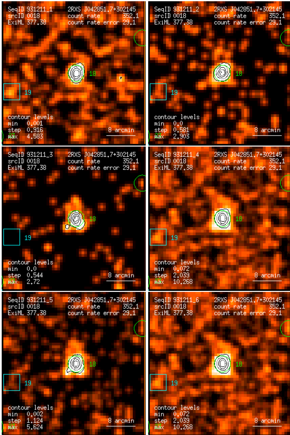
Figure 18: RASS 931211: detection 0018: band rate images, Gaussian filter: (1) PSPC channels 11 – 41, (2) 52 – 90, (3) 91 – 201, (4) 11 – 235, (5) 52 – 201, (6) 11 – 201. Broad band rates in counts/ks. Band rate contour levels in counts/ks/arcmin 2 .
