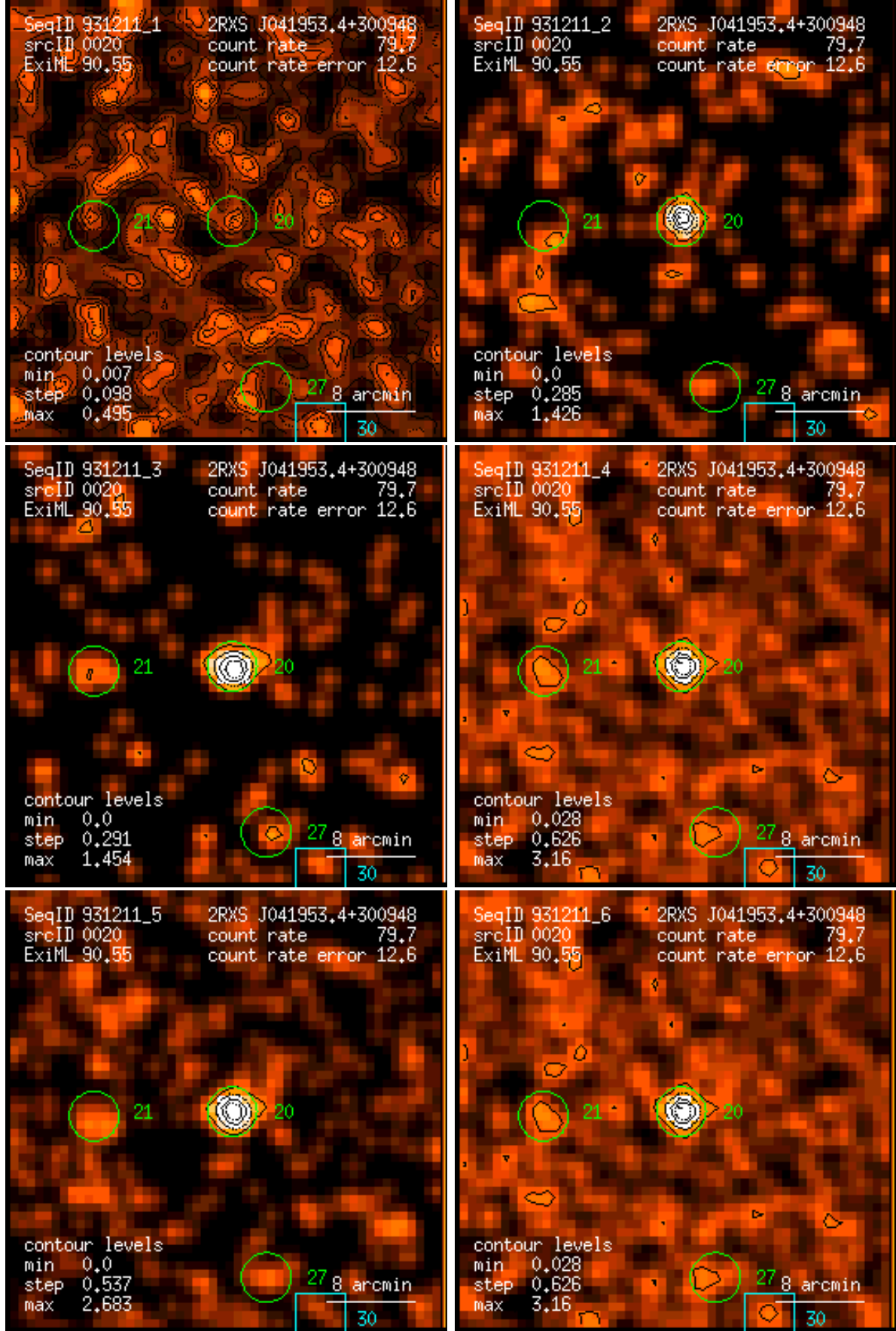
Figure 20: RASS 931211: detection 0020: band rate images, Gaussian filter: (1) PSPC channels 11 – 41, (2) 52 – 90, (3) 91 – 201, (4) 11 – 235, (5) 52 – 201, (6) 11 – 201. Broad band rates in counts/ks. Band rate contour levels in counts/ks/arcmin 2 .
