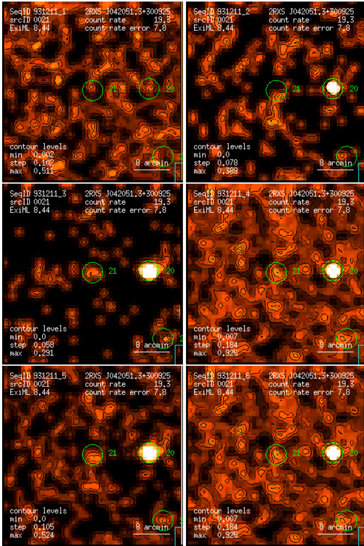
Figure 21: RASS 931211: detection 0021: band rate images, Gaussian filter: (1) PSPC channels 11 – 41, (2) 52 – 90, (3) 91 – 201, (4) 11 – 235, (5) 52 – 201, (6) 11 – 201. Broad band rates in counts/ks. Band rate contour levels in counts/ks/arcmin 2 .
