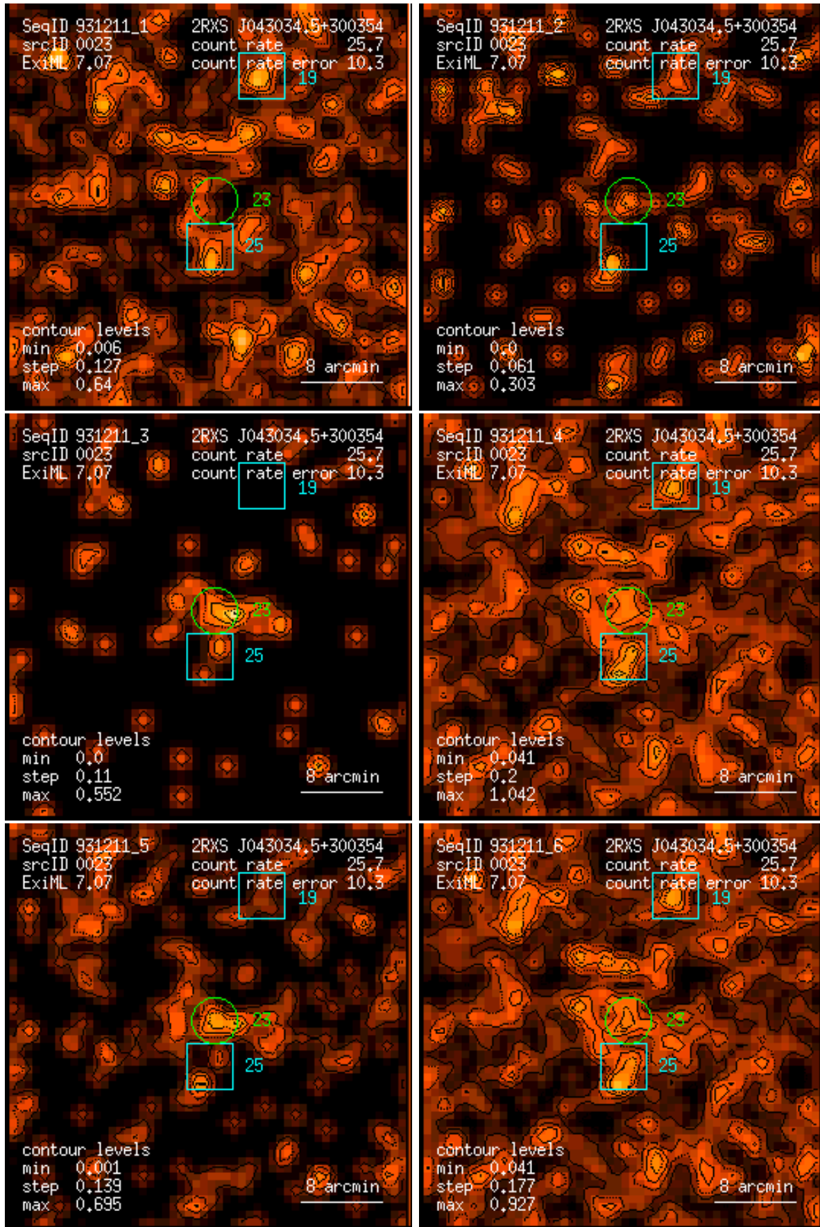
Figure 23: RASS 931211: detection 0023: band rate images, Gaussian filter: (1) PSPC channels 11 – 41, (2) 52 – 90, (3) 91 – 201, (4) 11 – 235, (5) 52 – 201, (6) 11 – 201. Broad band rates in counts/ks. Band rate contour levels in counts/ks/arcmin 2 .
