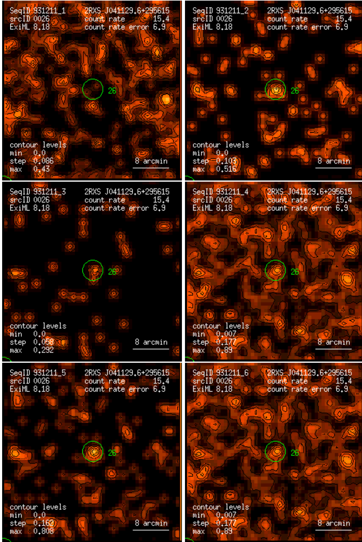
Figure 26: RASS 931211: detection 0026: band rate images, Gaussian filter: (1) PSPC channels 11 – 41, (2) 52 – 90, (3) 91 – 201, (4) 11 – 235, (5) 52 – 201, (6) 11 – 201. Broad band rates in counts/ks. Band rate contour levels in counts/ks/arcmin 2 .
