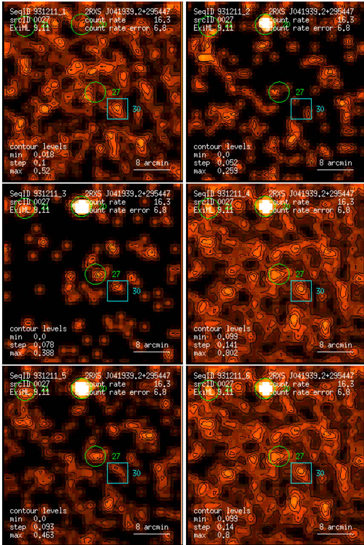
Figure 27: RASS 931211: detection 0027: band rate images, Gaussian filter: (1) PSPC channels 11 – 41, (2) 52 – 90, (3) 91 – 201, (4) 11 – 235, (5) 52 – 201, (6) 11 – 201. Broad band rates in counts/ks. Band rate contour levels in counts/ks/arcmin 2 .
