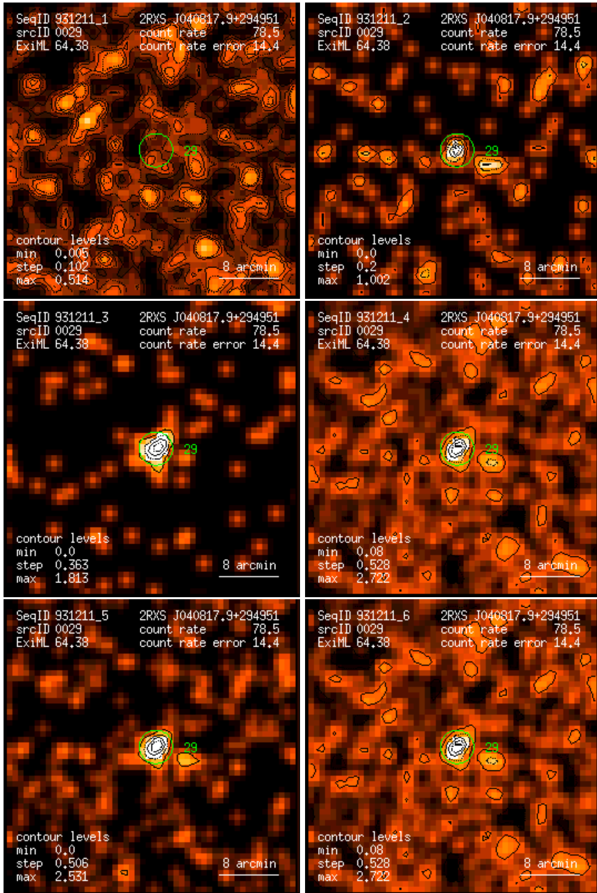
Figure 29: RASS 931211: detection 0029: band rate images, Gaussian filter: (1) PSPC channels 11 – 41, (2) 52 – 90, (3) 91 – 201, (4) 11 – 235, (5) 52 – 201, (6) 11 – 201. Broad band rates in counts/ks. Band rate contour levels in counts/ks/arcmin 2 .
