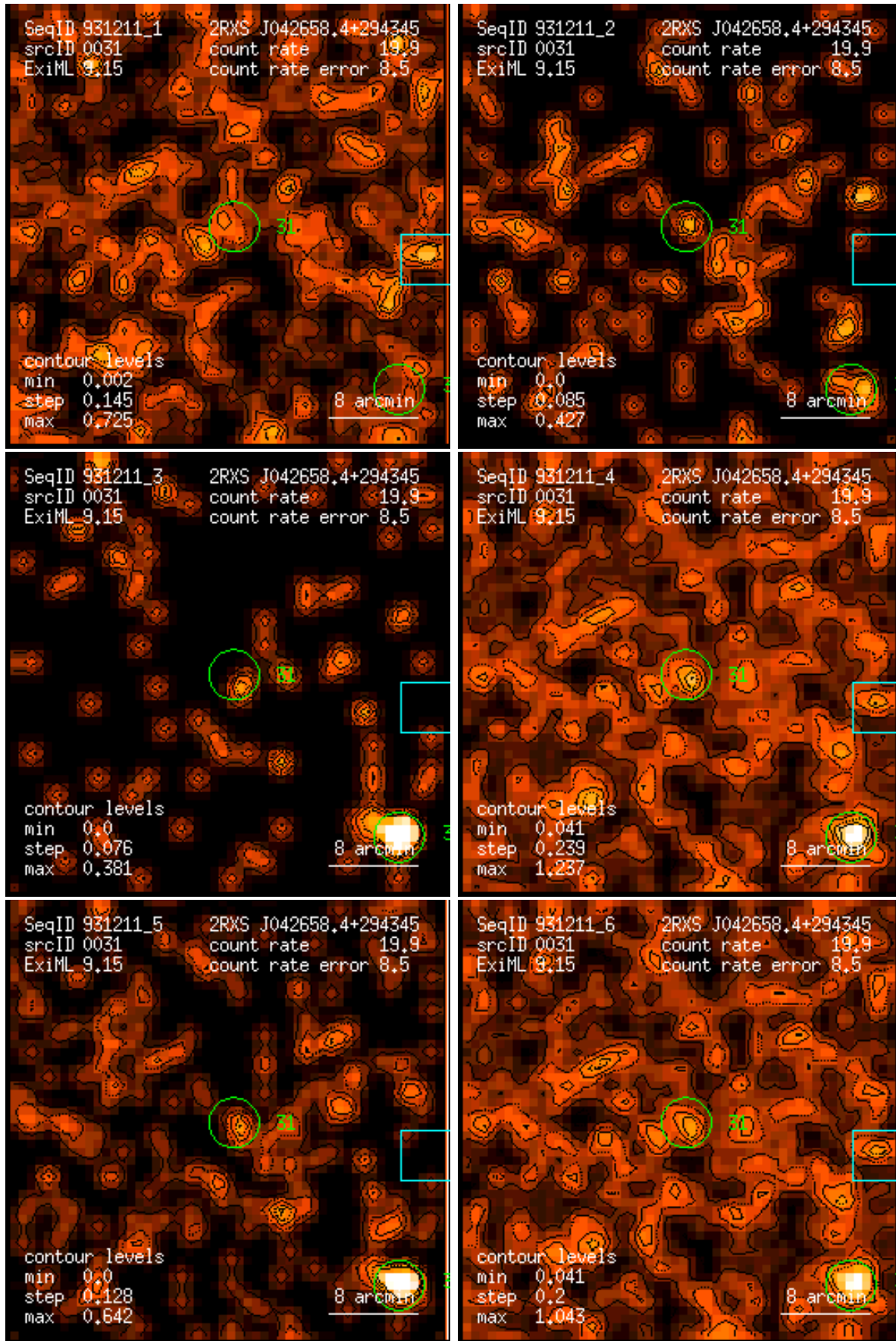
Figure 31: RASS 931211: detection 0031: band rate images, Gaussian filter: (1) PSPC channels 11 – 41, (2) 52 – 90, (3) 91 – 201, (4) 11 – 235, (5) 52 – 201, (6) 11 – 201. Broad band rates in counts/ks. Band rate contour levels in counts/ks/arcmin 2 .
