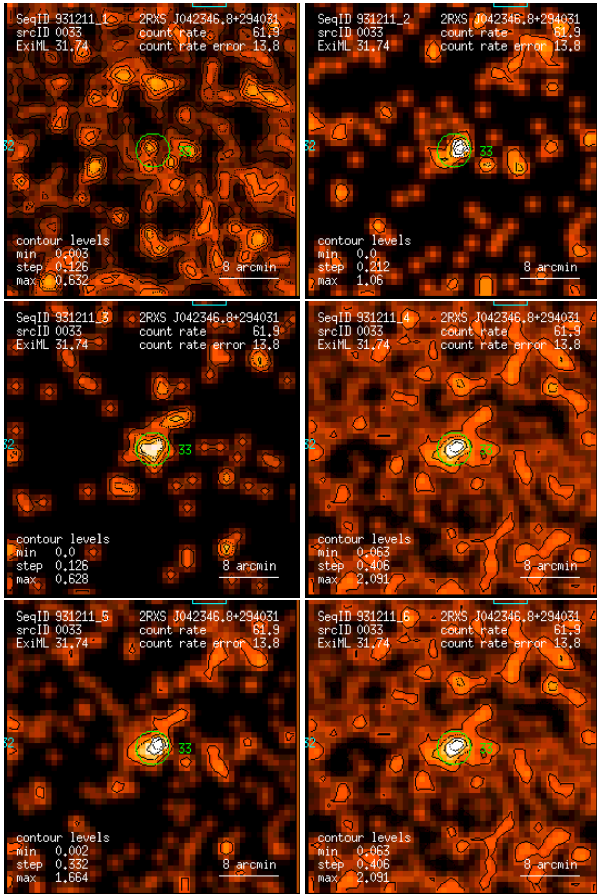
Figure 33: RASS 931211: detection 0033: band rate images, Gaussian filter: (1) PSPC channels 11 – 41, (2) 52 – 90, (3) 91 – 201, (4) 11 – 235, (5) 52 – 201, (6) 11 – 201. Broad band rates in counts/ks. Band rate contour levels in counts/ks/arcmin 2 .
