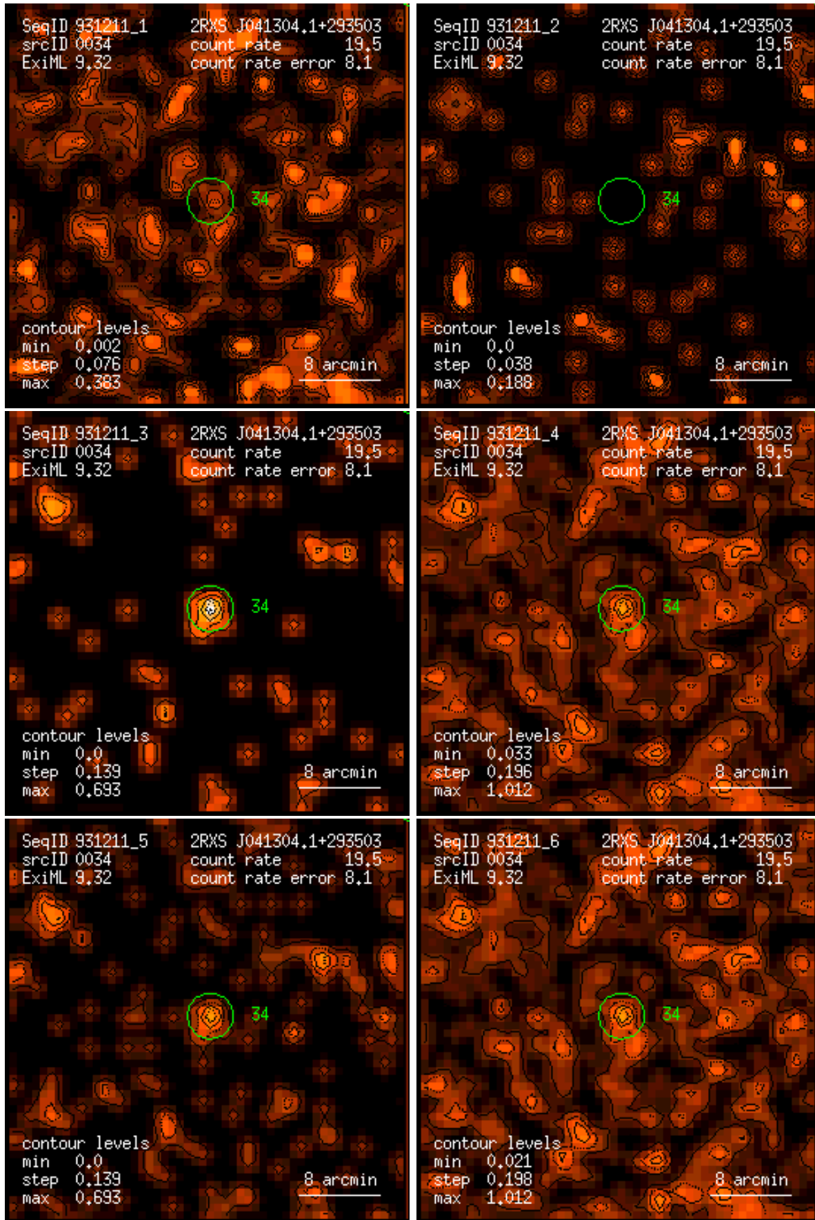
Figure 34: RASS 931211: detection 0034: band rate images, Gaussian filter: (1) PSPC channels 11 – 41, (2) 52 – 90, (3) 91 – 201, (4) 11 – 235, (5) 52 – 201, (6) 11 – 201. Broad band rates in counts/ks. Band rate contour levels in counts/ks/arcmin 2 .
