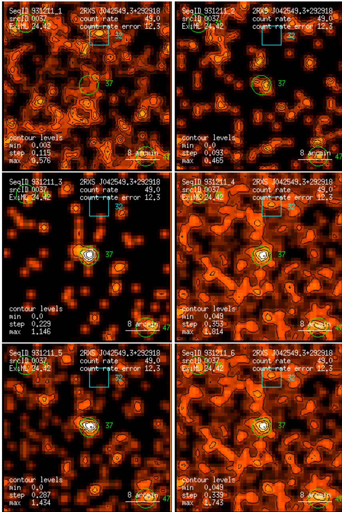
Figure 37: RASS 931211: detection 0037: band rate images, Gaussian filter: (1) PSPC channels 11 – 41, (2) 52 – 90, (3) 91 – 201, (4) 11 – 235, (5) 52 – 201, (6) 11 – 201. Broad band rates in counts/ks. Band rate contour levels in counts/ks/arcmin 2 .
