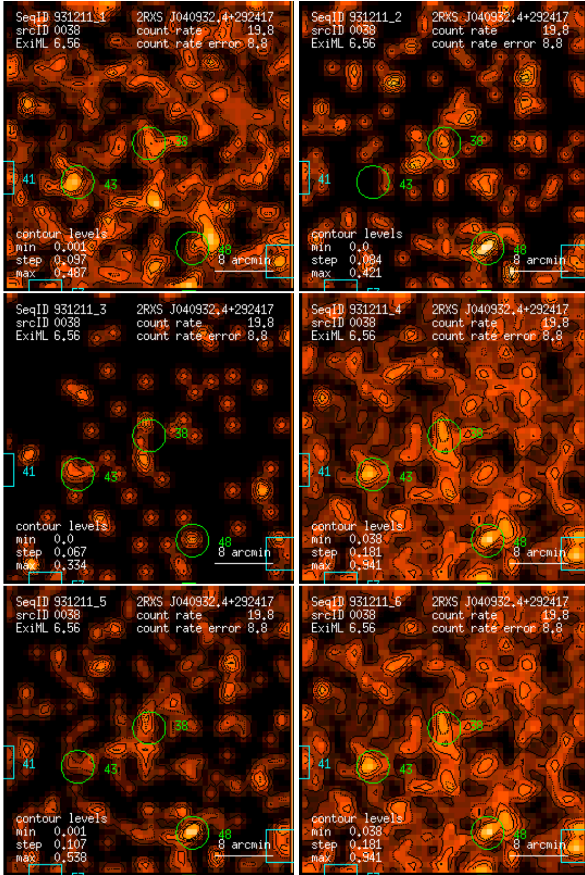
Figure 38: RASS 931211: detection 0038: band rate images, Gaussian filter: (1) PSPC channels 11 – 41, (2) 52 – 90, (3) 91 – 201, (4) 11 – 235, (5) 52 – 201, (6) 11 – 201. Broad band rates in counts/ks. Band rate contour levels in counts/ks/arcmin 2 .
