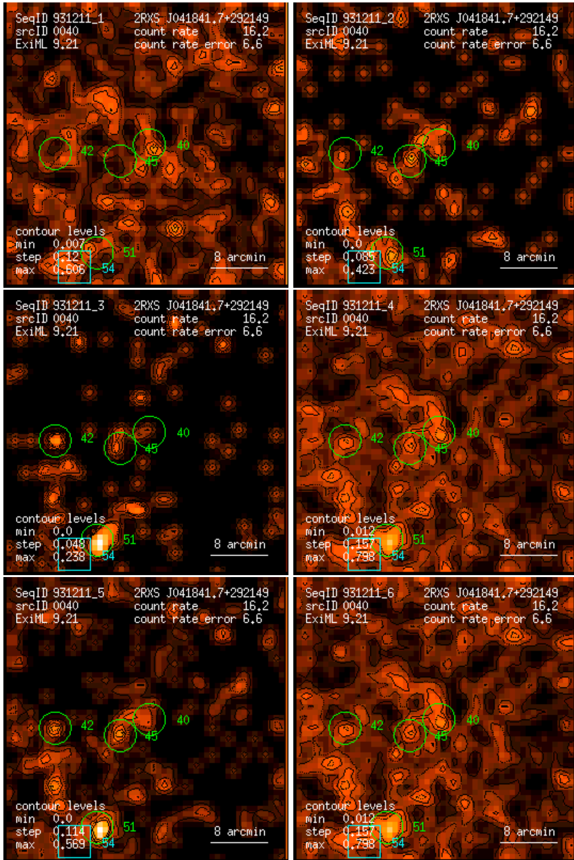
Figure 40: RASS 931211: detection 0040: band rate images, Gaussian filter: (1) PSPC channels 11 – 41, (2) 52 – 90, (3) 91 – 201, (4) 11 – 235, (5) 52 – 201, (6) 11 – 201. Broad band rates in counts/ks. Band rate contour levels in counts/ks/arcmin 2 .
