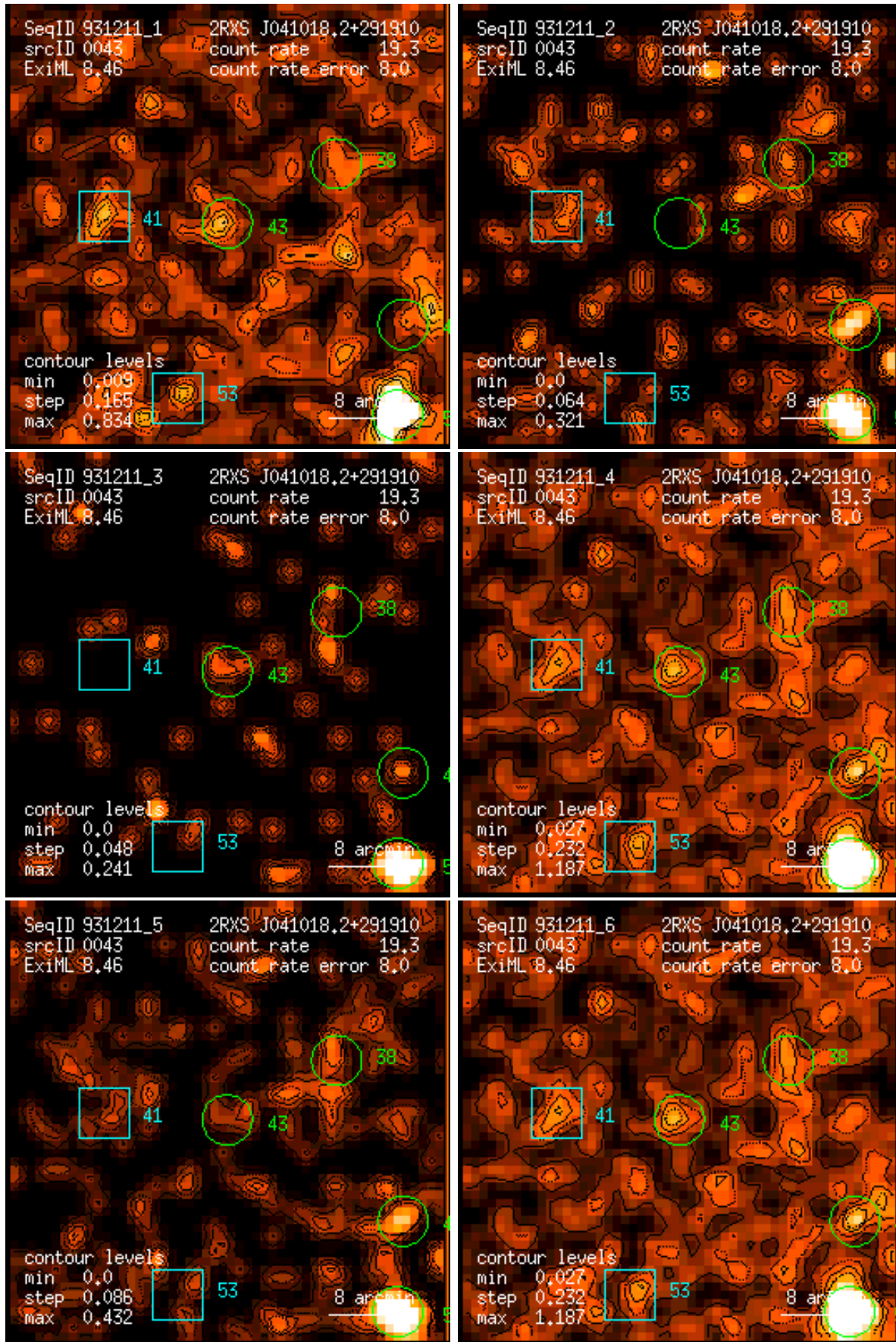
Figure 43: RASS 931211: detection 0043: band rate images, Gaussian filter: (1) PSPC channels 11 – 41, (2) 52 – 90, (3) 91 – 201, (4) 11 – 235, (5) 52 – 201, (6) 11 – 201. Broad band rates in counts/ks. Band rate contour levels in counts/ks/arcmin 2 .
