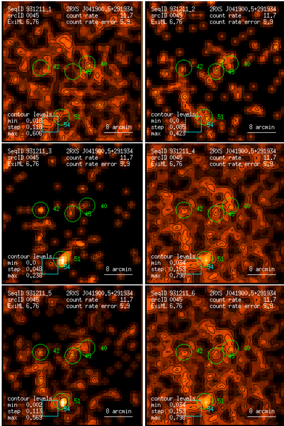
Figure 45: RASS 931211: detection 0045: band rate images, Gaussian filter: (1) PSPC channels 11 – 41, (2) 52 – 90, (3) 91 – 201, (4) 11 – 235, (5) 52 – 201, (6) 11 – 201. Broad band rates in counts/ks. Band rate contour levels in counts/ks/arcmin 2 .
