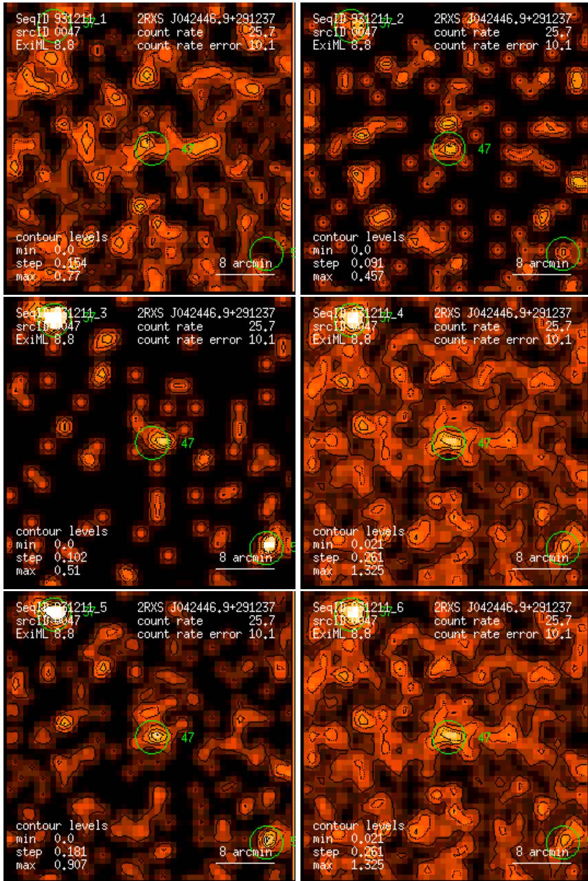
Figure 47: RASS 931211: detection 0047: band rate images, Gaussian filter: (1) PSPC channels 11 – 41, (2) 52 – 90, (3) 91 – 201, (4) 11 – 235, (5) 52 – 201, (6) 11 – 201. Broad band rates in counts/ks. Band rate contour levels in counts/ks/arcmin 2 .
