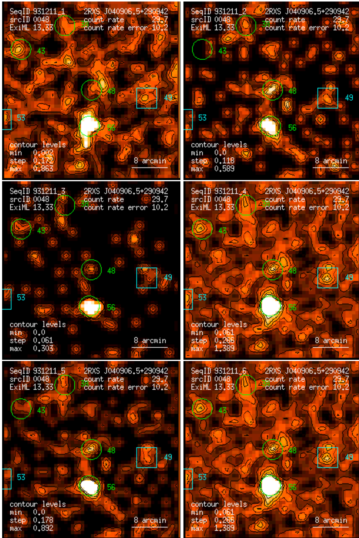
Figure 48: RASS 931211: detection 0048: band rate images, Gaussian filter: (1) PSPC channels 11 – 41, (2) 52 – 90, (3) 91 – 201, (4) 11 – 235, (5) 52 – 201, (6) 11 – 201. Broad band rates in counts/ks. Band rate contour levels in counts/ks/arcmin 2 .
