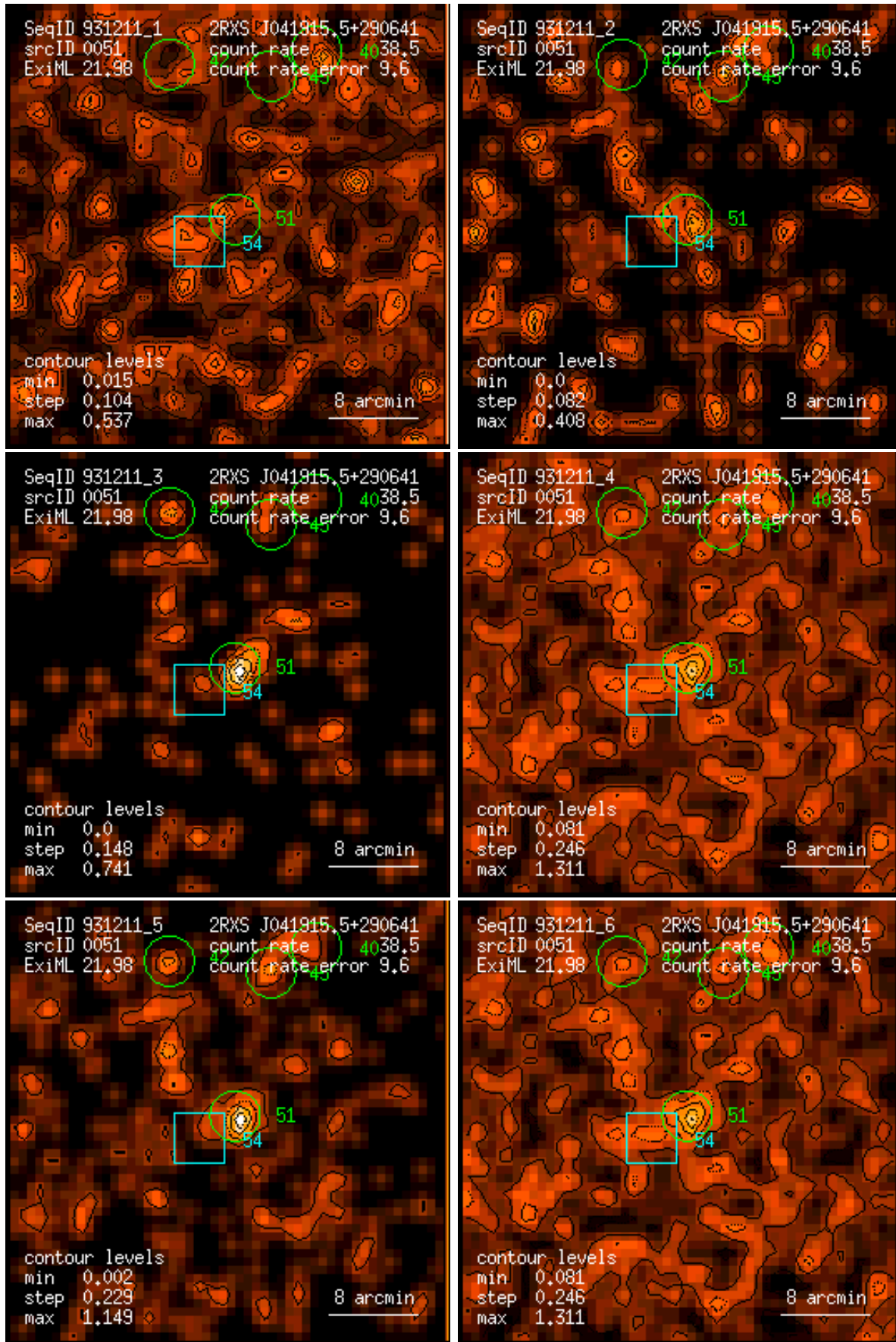
Figure 51: RASS 931211: detection 0051: band rate images, Gaussian filter: (1) PSPC channels 11 – 41, (2) 52 – 90, (3) 91 – 201, (4) 11 – 235, (5) 52 – 201, (6) 11 – 201. Broad band rates in counts/ks. Band rate contour levels in counts/ks/arcmin 2 .
