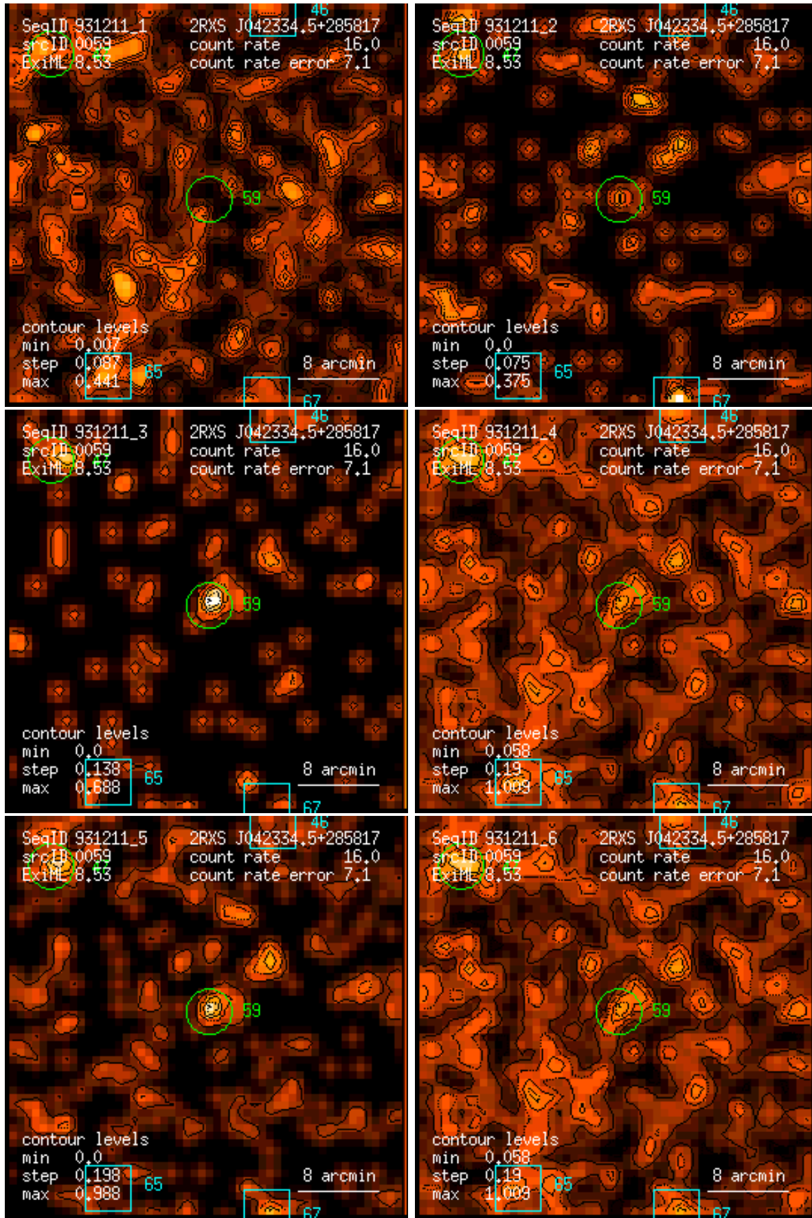
Figure 59: RASS 931211: detection 0059: band rate images, Gaussian filter: (1) PSPC channels 11 – 41, (2) 52 – 90, (3) 91 – 201, (4) 11 – 235, (5) 52 – 201, (6) 11 – 201. Broad band rates in counts/ks. Band rate contour levels in counts/ks/arcmin 2 .
