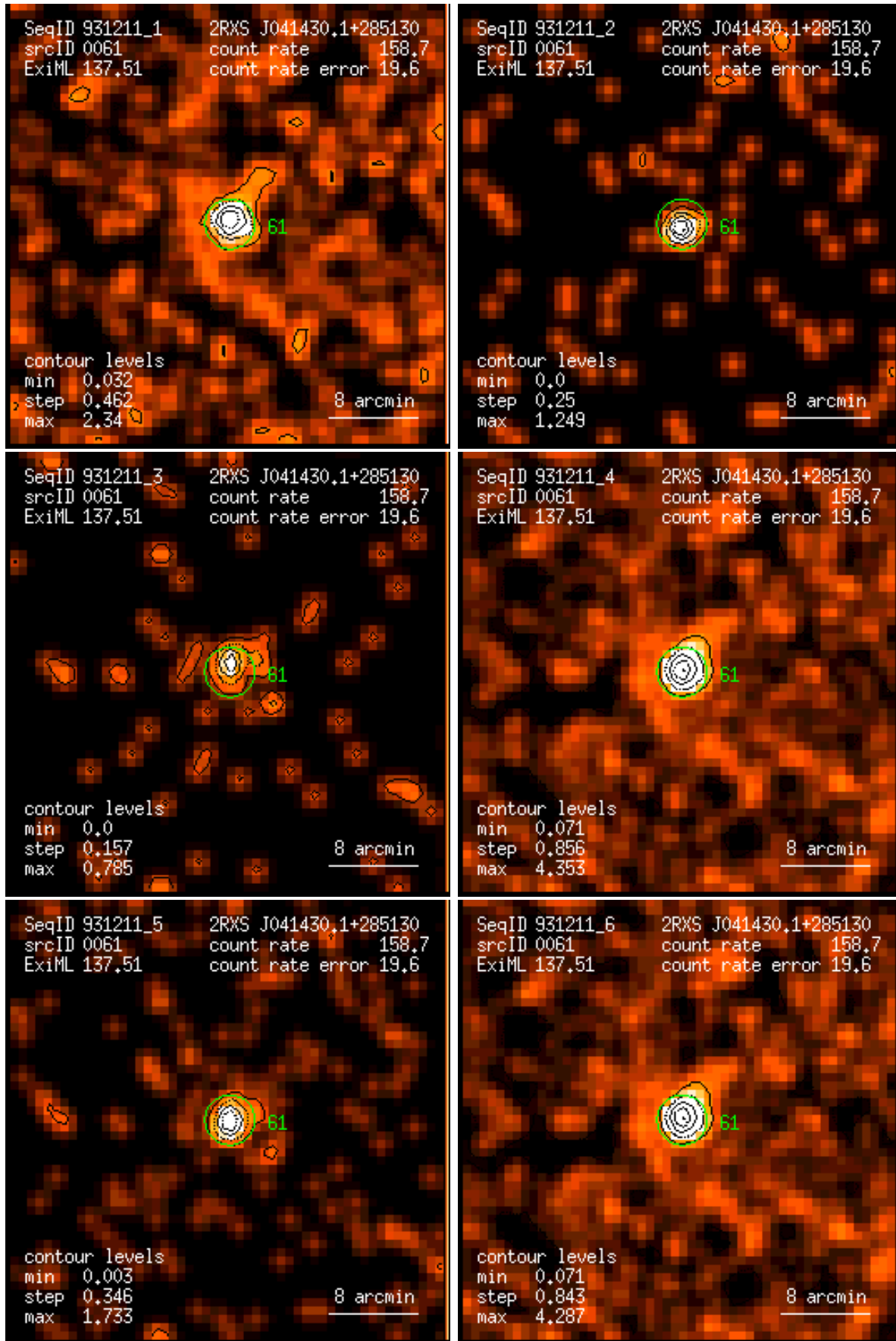
Figure 61: RASS 931211: detection 0061: band rate images, Gaussian filter: (1) PSPC channels 11 – 41, (2) 52 – 90, (3) 91 – 201, (4) 11 – 235, (5) 52 – 201, (6) 11 – 201. Broad band rates in counts/ks. Band rate contour levels in counts/ks/arcmin 2 .
