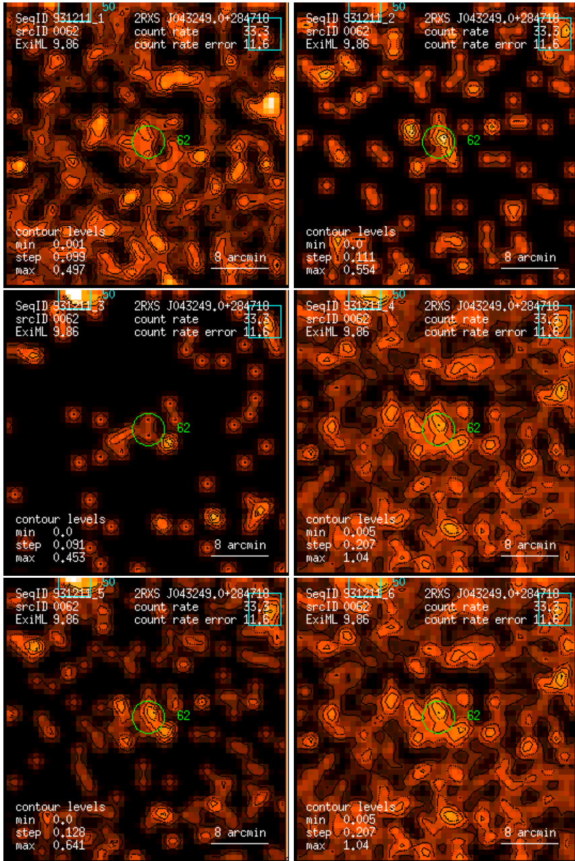
Figure 62: RASS 931211: detection 0062: band rate images, Gaussian filter: (1) PSPC channels 11 – 41, (2) 52 – 90, (3) 91 – 201, (4) 11 – 235, (5) 52 – 201, (6) 11 – 201. Broad band rates in counts/ks. Band rate contour levels in counts/ks/arcmin 2 .
