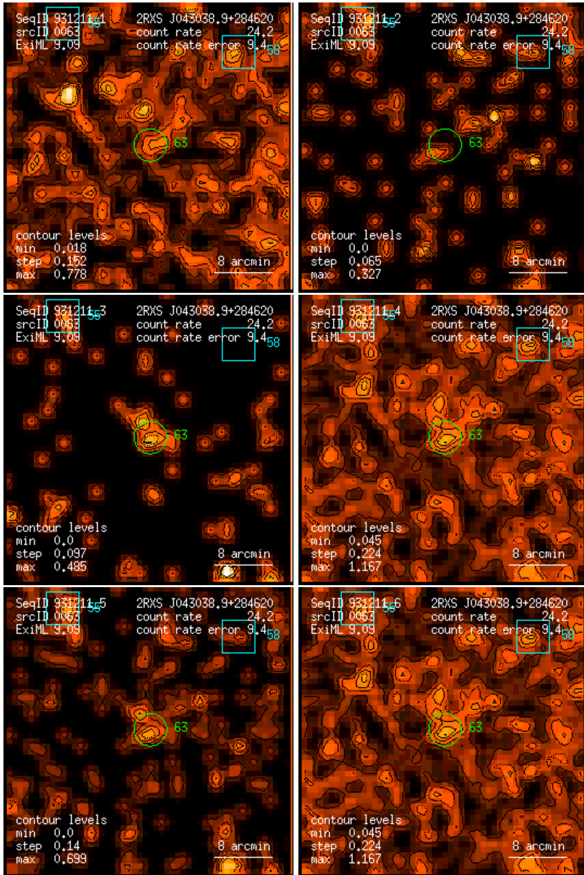
Figure 63: RASS 931211: detection 0063: band rate images, Gaussian filter: (1) PSPC channels 11 – 41, (2) 52 – 90, (3) 91 – 201, (4) 11 – 235, (5) 52 – 201, (6) 11 – 201. Broad band rates in counts/ks. Band rate contour levels in counts/ks/arcmin 2 .
