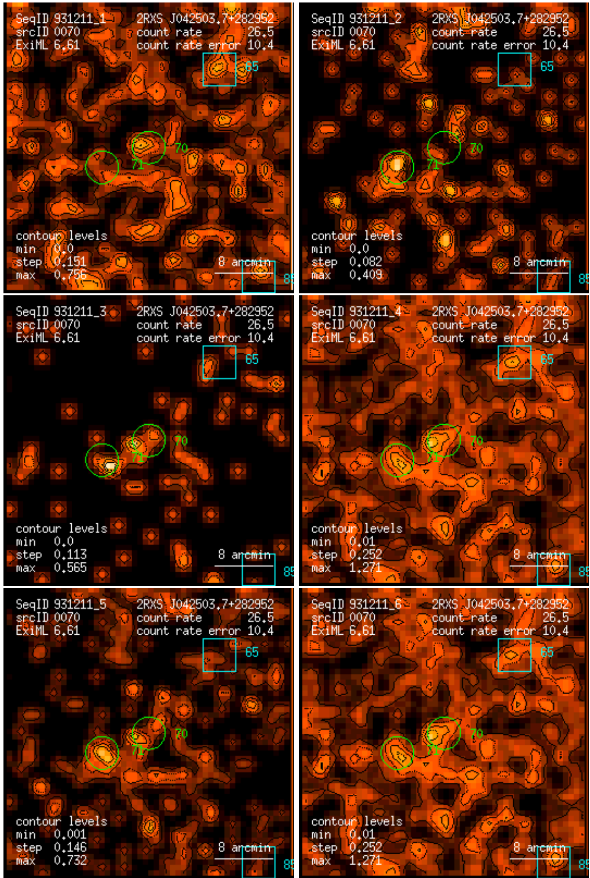
Figure 70: RASS 931211: detection 0070: band rate images, Gaussian filter: (1) PSPC channels 11 – 41, (2) 52 – 90, (3) 91 – 201, (4) 11 – 235, (5) 52 – 201, (6) 11 – 201. Broad band rates in counts/ks. Band rate contour levels in counts/ks/arcmin 2 .
