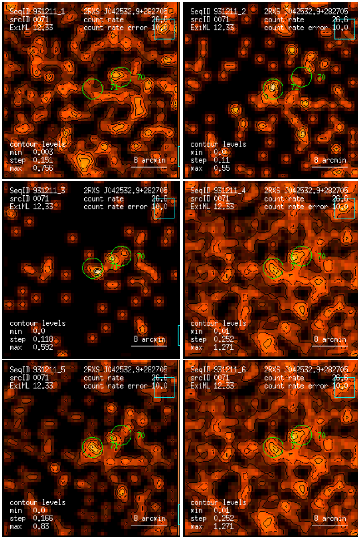
Figure 71: RASS 931211: detection 0071: band rate images, Gaussian filter: (1) PSPC channels 11 – 41, (2) 52 – 90, (3) 91 – 201, (4) 11 – 235, (5) 52 – 201, (6) 11 – 201. Broad band rates in counts/ks. Band rate contour levels in counts/ks/arcmin 2 .
