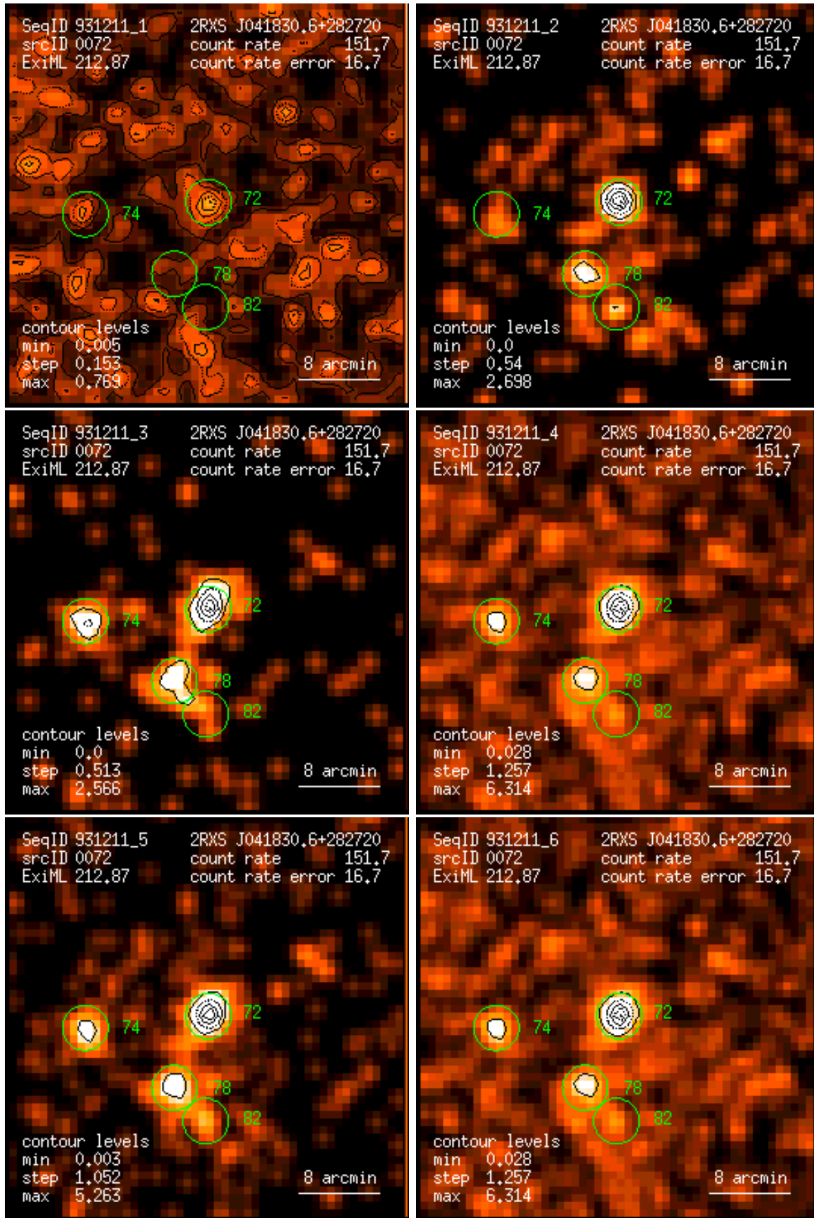
Figure 72: RASS 931211: detection 0072: band rate images, Gaussian filter: (1) PSPC channels 11 – 41, (2) 52 – 90, (3) 91 – 201, (4) 11 – 235, (5) 52 – 201, (6) 11 – 201. Broad band rates in counts/ks. Band rate contour levels in counts/ks/arcmin 2 .
