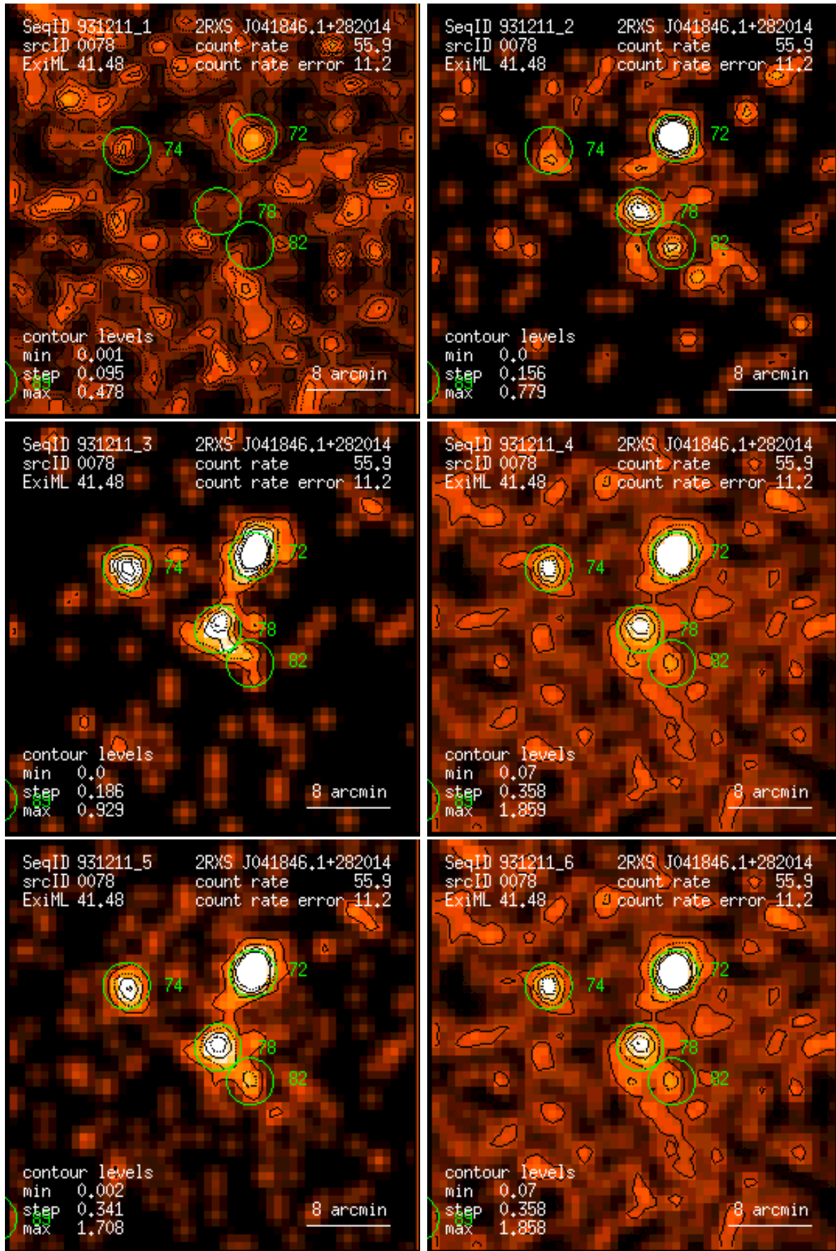
Figure 78: RASS 931211: detection 0078: band rate images, Gaussian filter: (1) PSPC channels 11 – 41, (2) 52 – 90, (3) 91 – 201, (4) 11 – 235, (5) 52 – 201, (6) 11 – 201. Broad band rates in counts/ks. Band rate contour levels in counts/ks/arcmin 2 .
