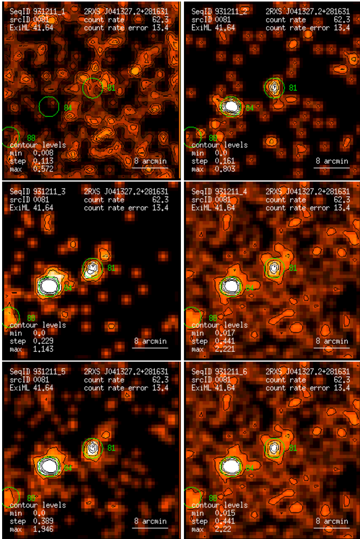
Figure 81: RASS 931211: detection 0081: band rate images, Gaussian filter: (1) PSPC channels 11 – 41, (2) 52 – 90, (3) 91 – 201, (4) 11 – 235, (5) 52 – 201, (6) 11 – 201. Broad band rates in counts/ks. Band rate contour levels in counts/ks/arcmin 2 .
