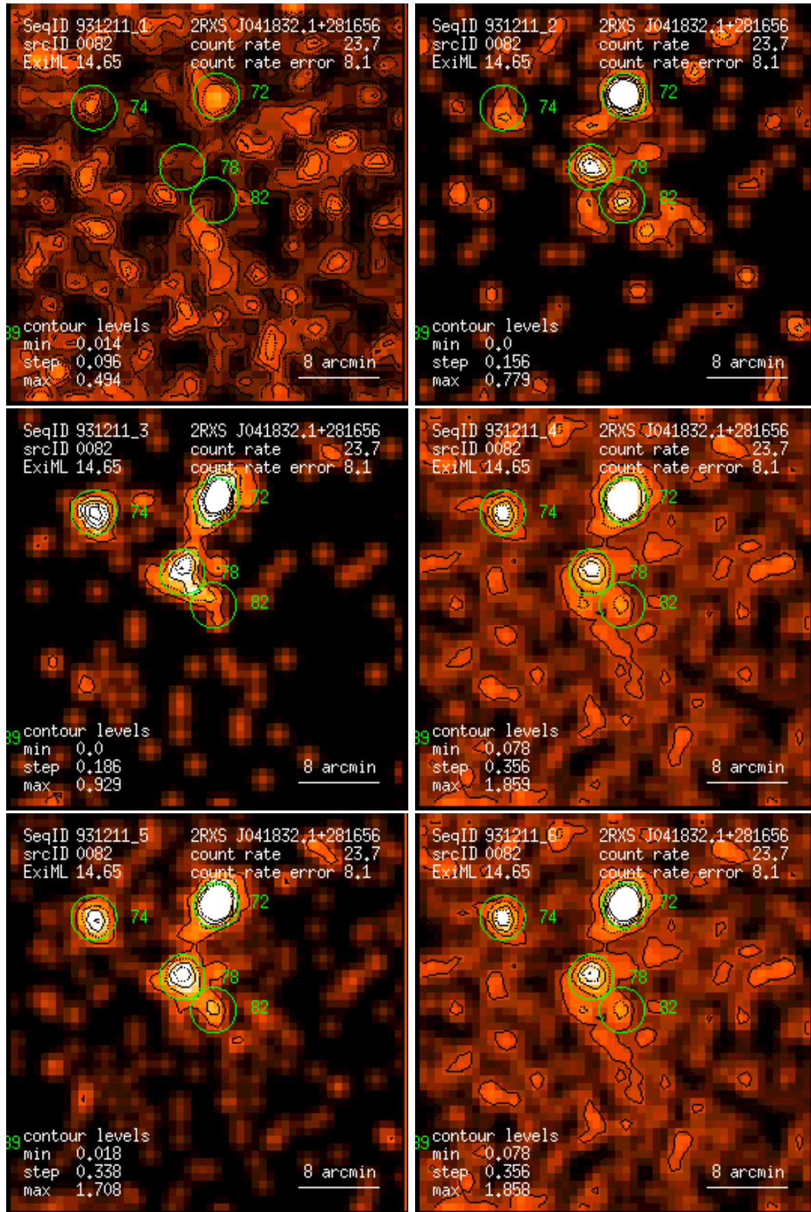
Figure 82: RASS 931211: detection 0082: band rate images, Gaussian filter: (1) PSPC channels 11 – 41, (2) 52 – 90, (3) 91 – 201, (4) 11 – 235, (5) 52 – 201, (6) 11 – 201. Broad band rates in counts/ks. Band rate contour levels in counts/ks/arcmin 2 .
