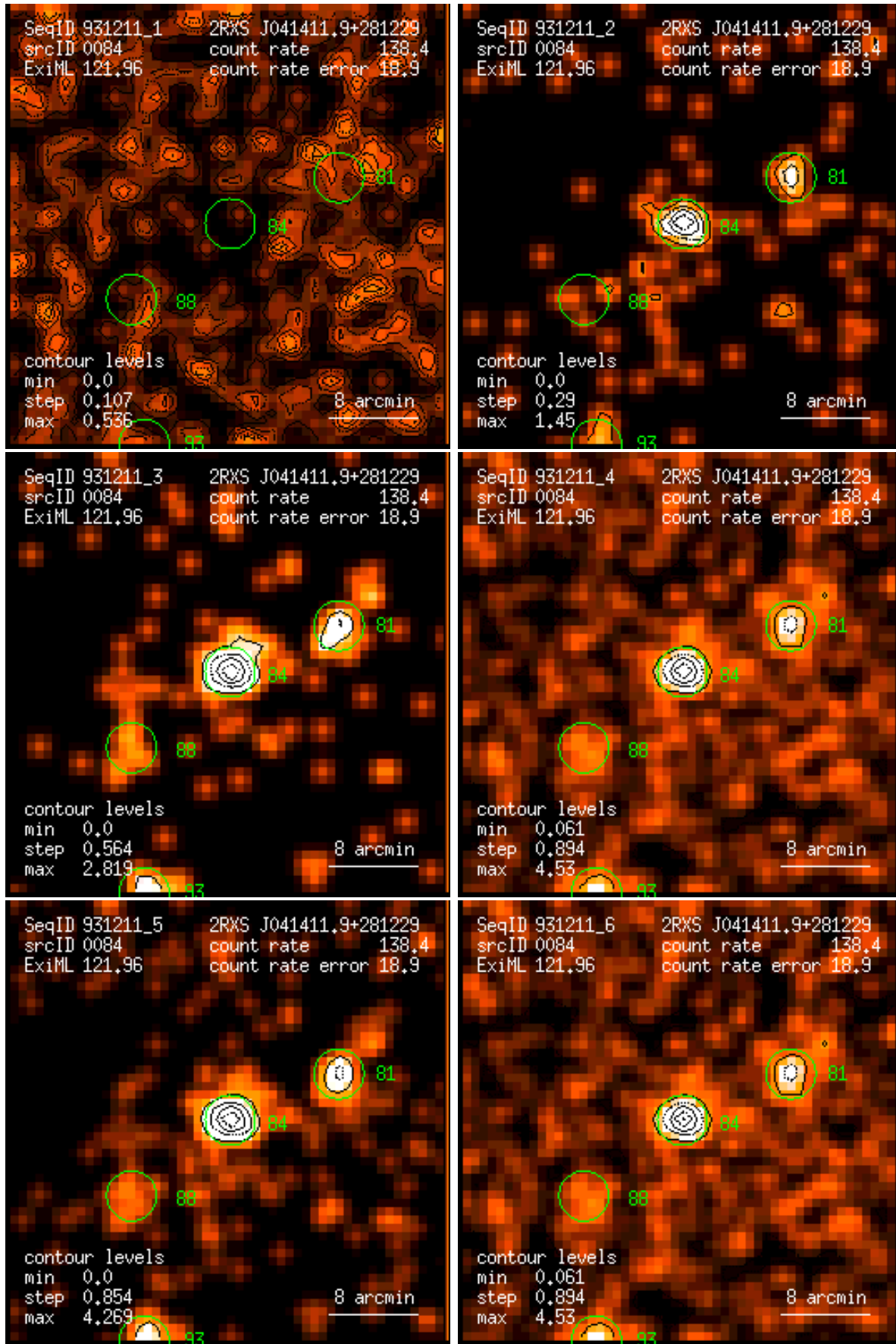
Figure 84: RASS 931211: detection 0084: band rate images, Gaussian filter: (1) PSPC channels 11 – 41, (2) 52 – 90, (3) 91 – 201, (4) 11 – 235, (5) 52 – 201, (6) 11 – 201. Broad band rates in counts/ks. Band rate contour levels in counts/ks/arcmin 2 .
