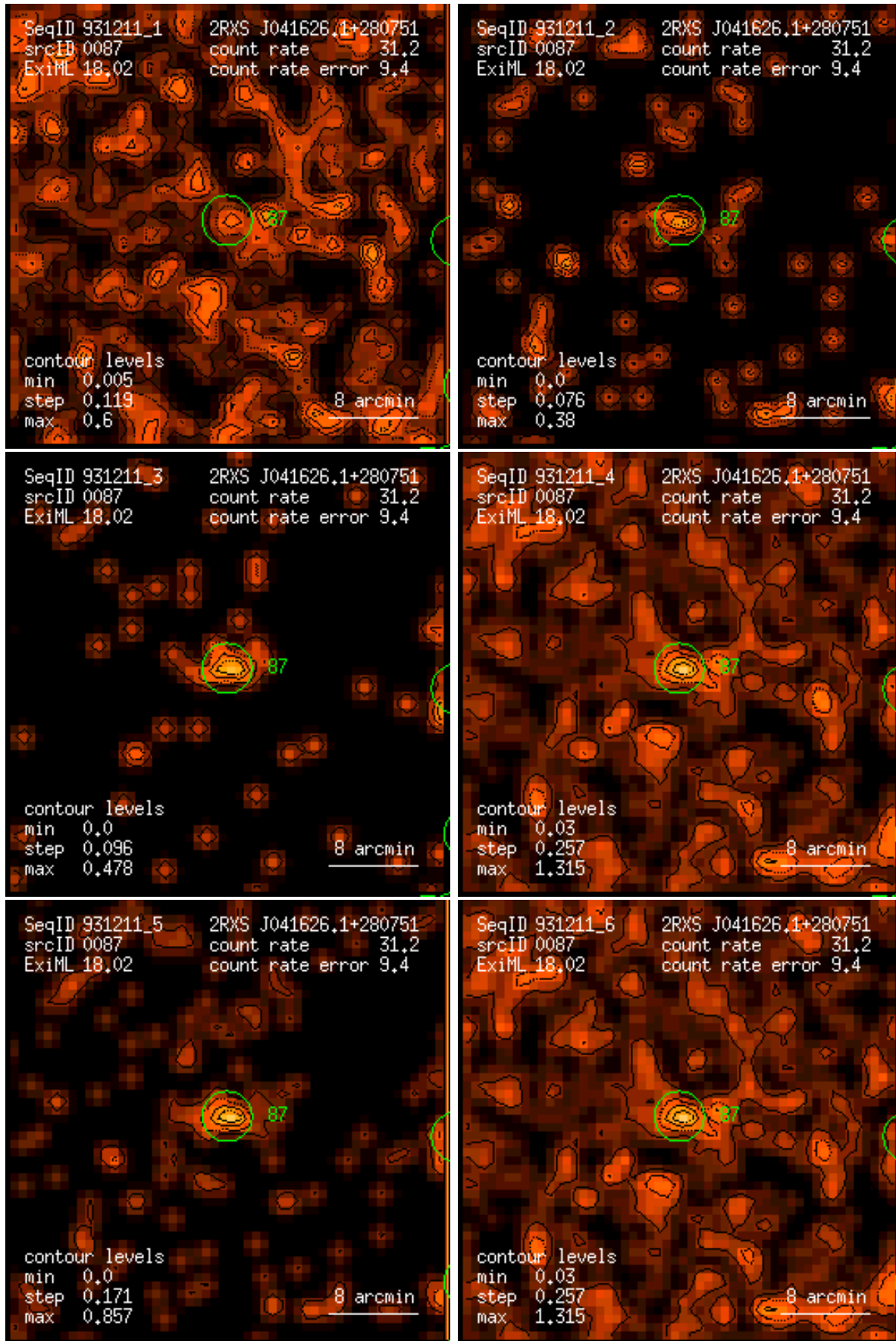
Figure 87: RASS 931211: detection 0087: band rate images, Gaussian filter: (1) PSPC channels 11 – 41, (2) 52 – 90, (3) 91 – 201, (4) 11 – 235, (5) 52 – 201, (6) 11 – 201. Broad band rates in counts/ks. Band rate contour levels in counts/ks/arcmin 2 .
