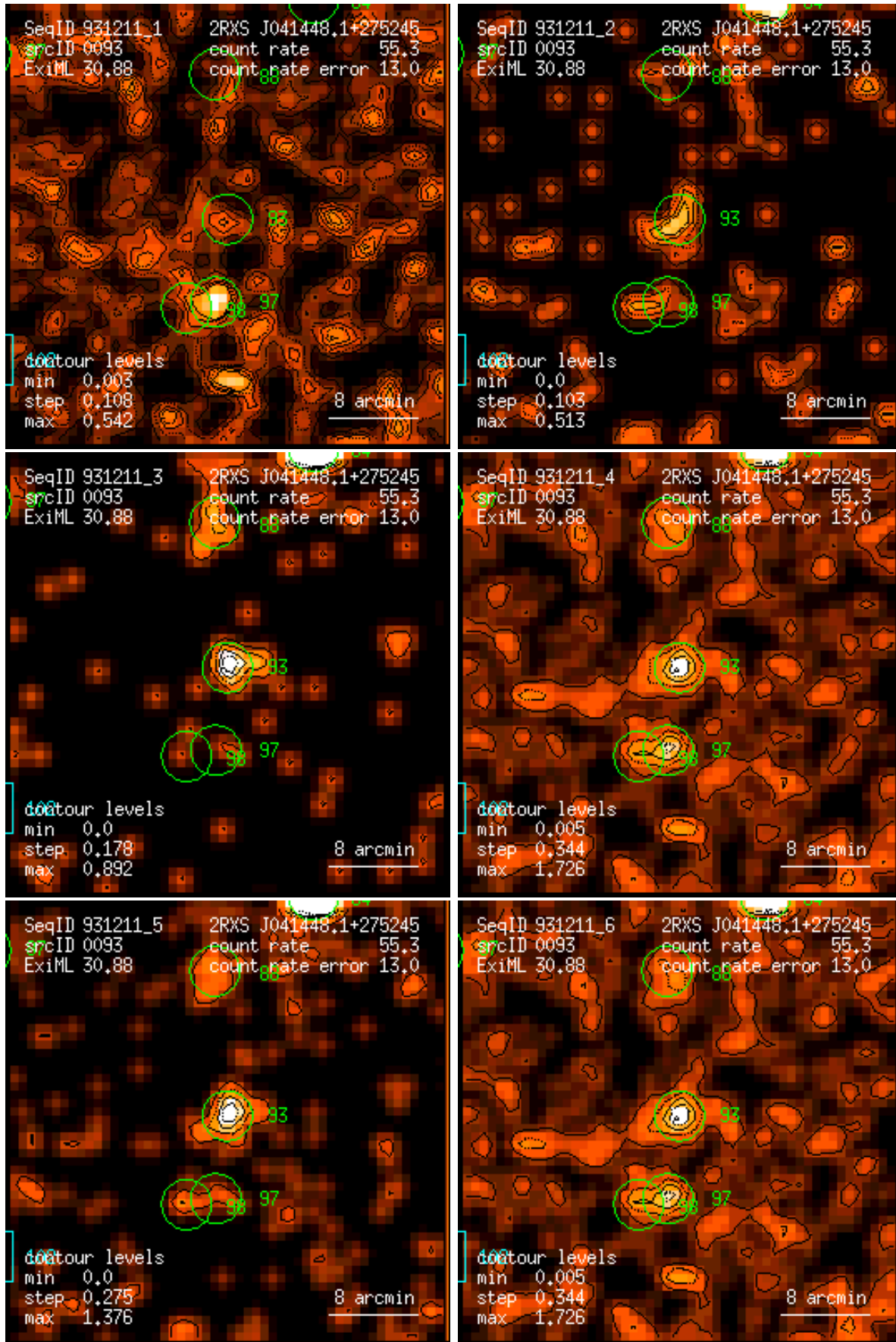
Figure 93: RASS 931211: detection 0093: band rate images, Gaussian filter: (1) PSPC channels 11 – 41, (2) 52 – 90, (3) 91 – 201, (4) 11 – 235, (5) 52 – 201, (6) 11 – 201. Broad band rates in counts/ks. Band rate contour levels in counts/ks/arcmin 2 .
