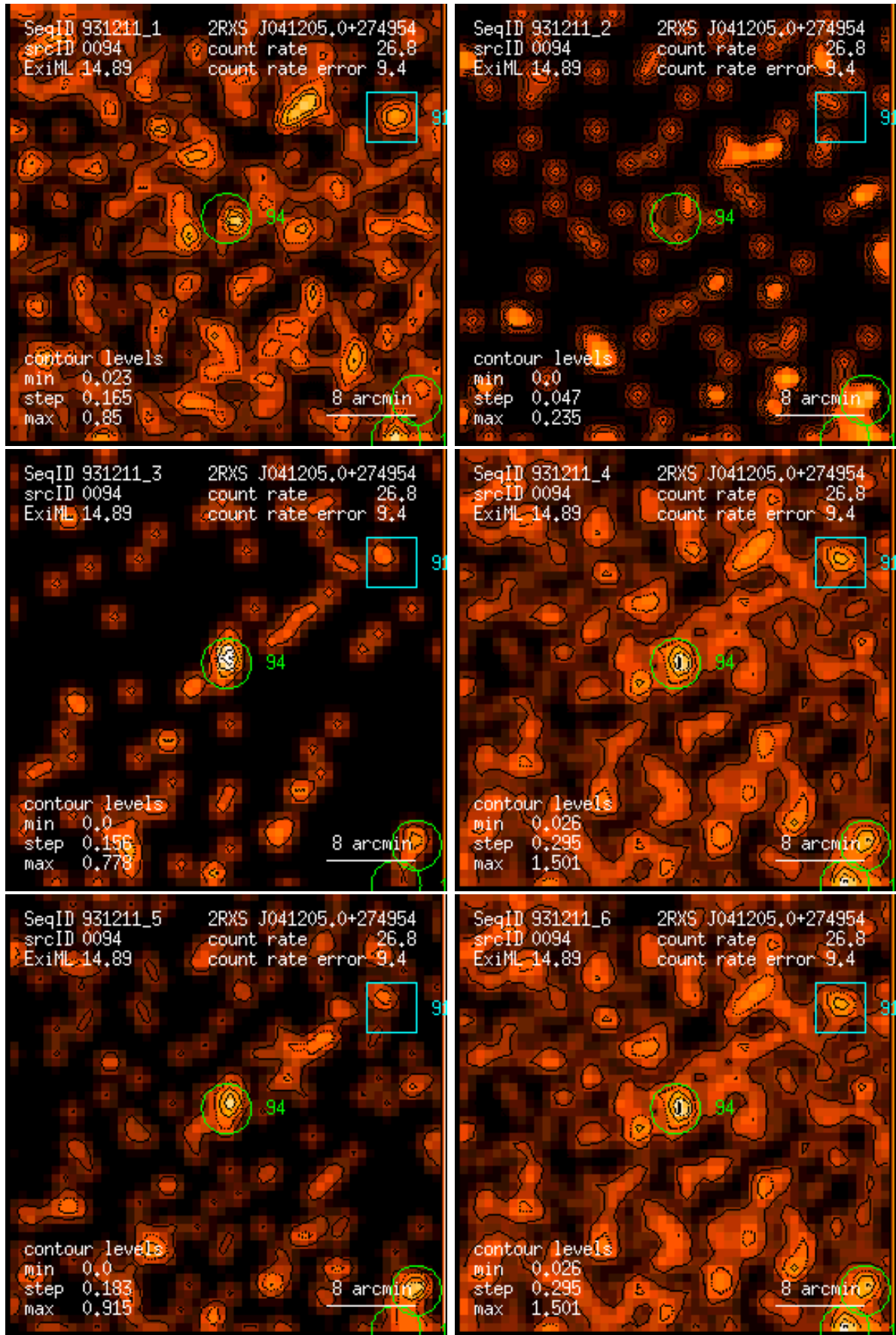
Figure 94: RASS 931211: detection 0094: band rate images, Gaussian filter: (1) PSPC channels 11 – 41, (2) 52 – 90, (3) 91 – 201, (4) 11 – 235, (5) 52 – 201, (6) 11 – 201. Broad band rates in counts/ks. Band rate contour levels in counts/ks/arcmin 2 .
