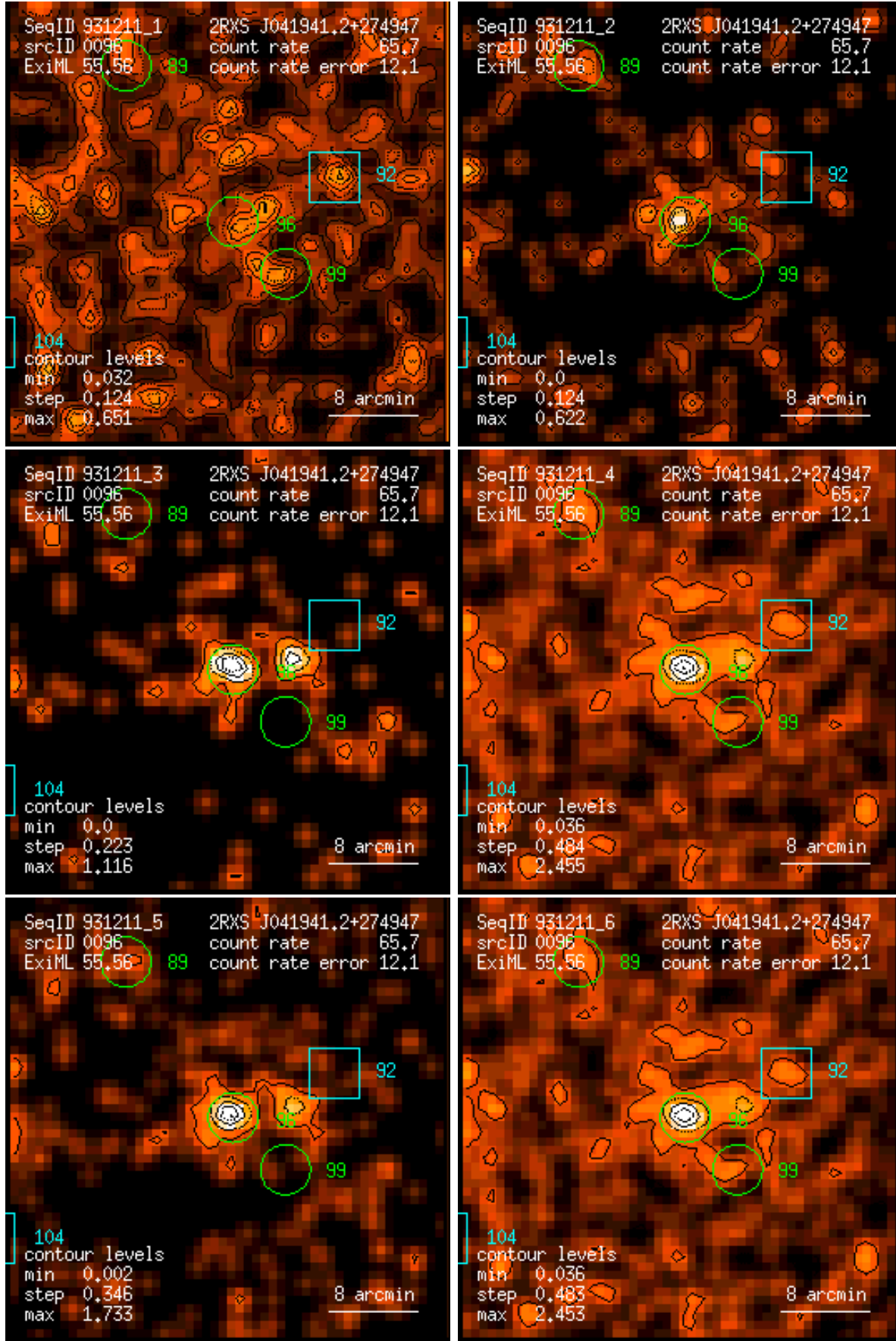
Figure 96: RASS 931211: detection 0096: band rate images, Gaussian filter: (1) PSPC channels 11 – 41, (2) 52 – 90, (3) 91 – 201, (4) 11 – 235, (5) 52 – 201, (6) 11 – 201. Broad band rates in counts/ks. Band rate contour levels in counts/ks/arcmin 2 .
