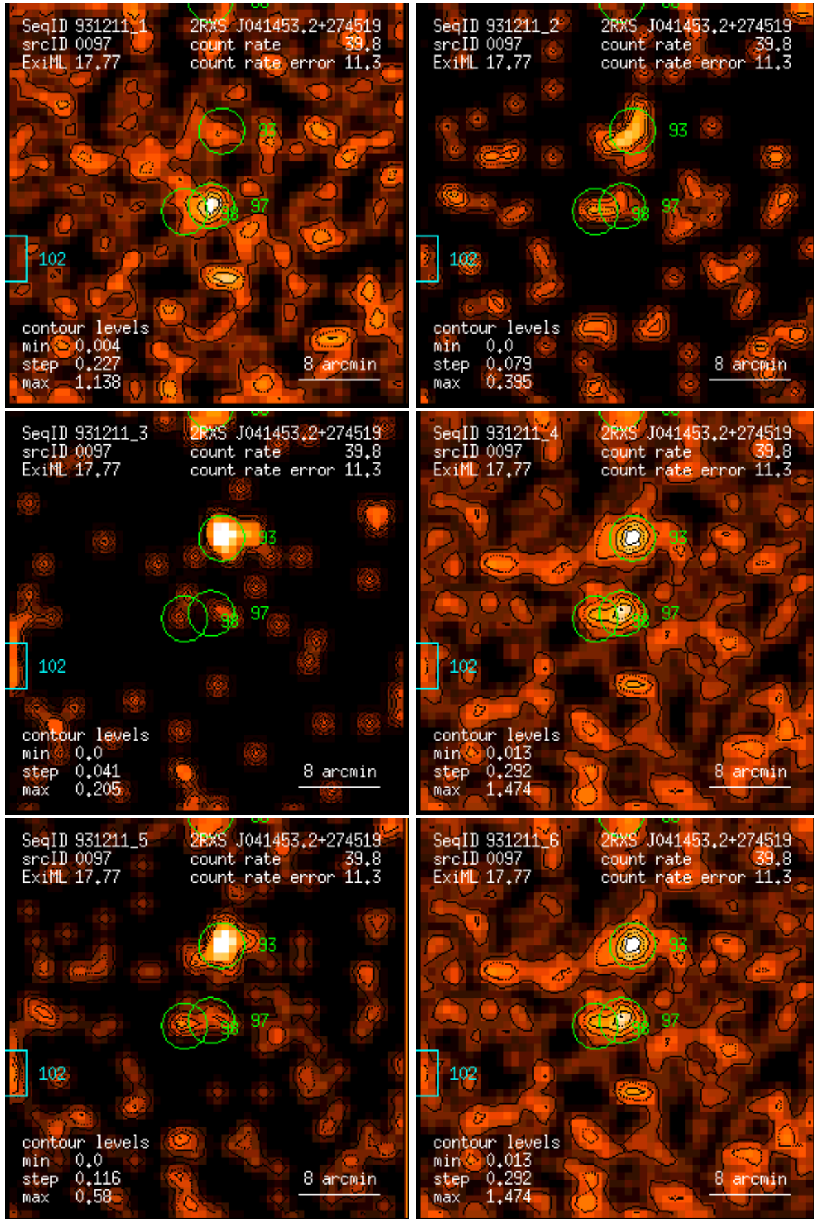
Figure 97: RASS 931211: detection 0097: band rate images, Gaussian filter: (1) PSPC channels 11 – 41, (2) 52 – 90, (3) 91 – 201, (4) 11 – 235, (5) 52 – 201, (6) 11 – 201. Broad band rates in counts/ks. Band rate contour levels in counts/ks/arcmin 2 .
