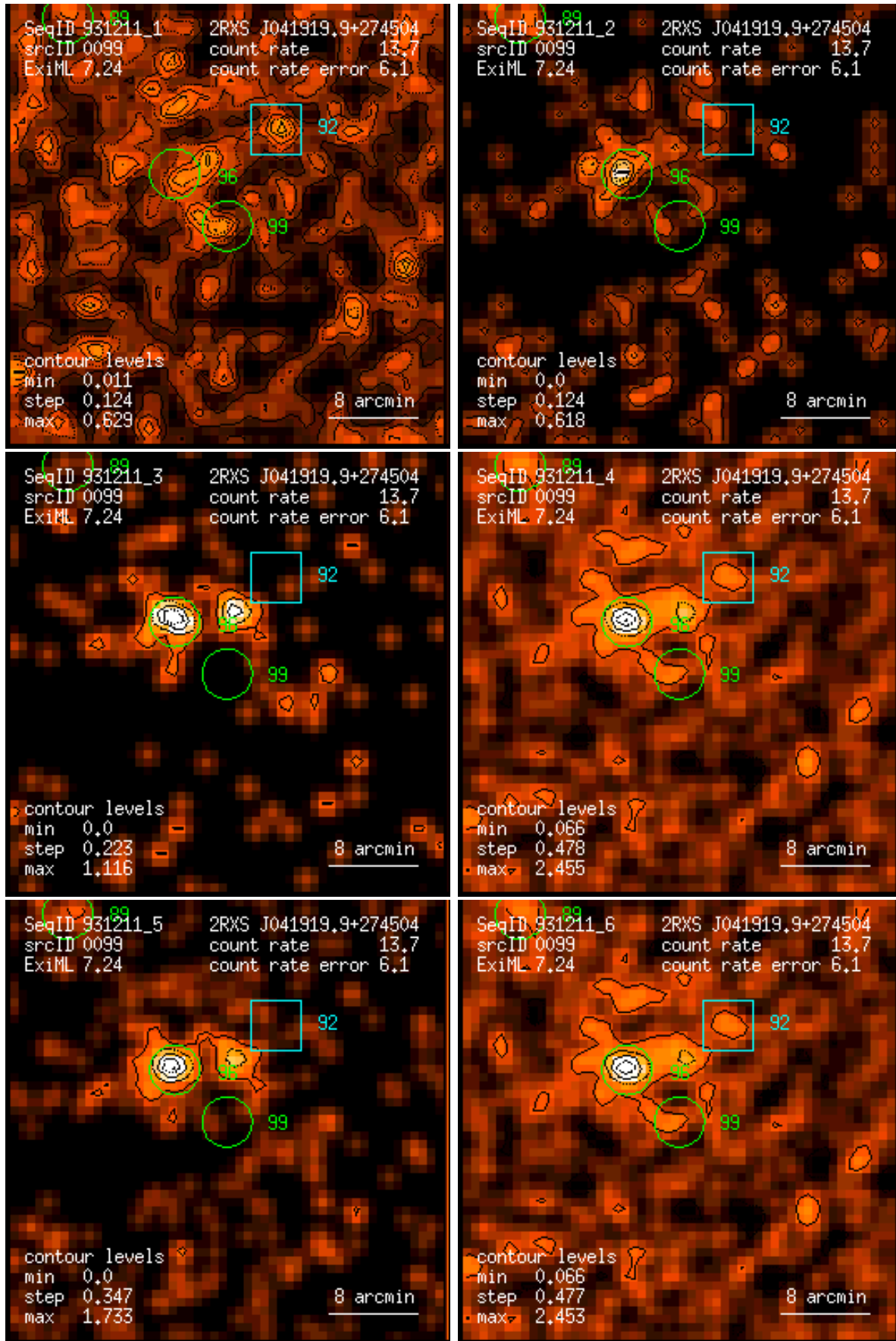
Figure 99: RASS 931211: detection 0099: band rate images, Gaussian filter: (1) PSPC channels 11 – 41, (2) 52 – 90, (3) 91 – 201, (4) 11 – 235, (5) 52 – 201, (6) 11 – 201. Broad band rates in counts/ks. Band rate contour levels in counts/ks/arcmin 2 .
