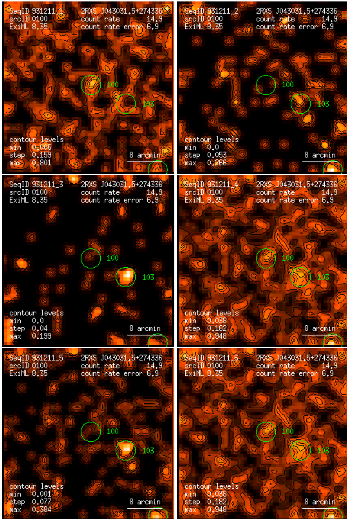
Figure 100: RASS 931211: detection 0100: band rate images, Gaussian filter: (1) PSPC channels 11 – 41, (2) 52 – 90, (3) 91 – 201, (4) 11 – 235, (5) 52 – 201, (6) 11 – 201. Broad band rates in counts/ks. Band rate contour levels in counts/ks/arcmin 2 .
