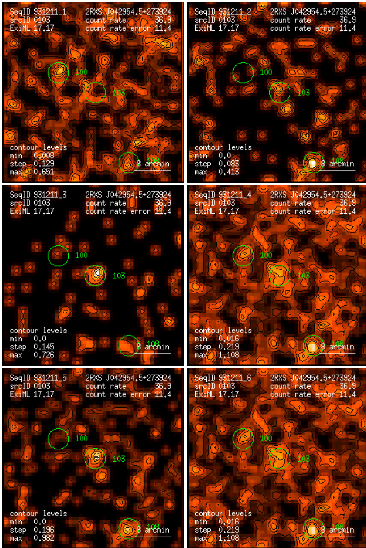
Figure 103: RASS 931211: detection 0103: band rate images, Gaussian filter: (1) PSPC channels 11 – 41, (2) 52 – 90, (3) 91 – 201, (4) 11 – 235, (5) 52 – 201, (6) 11 – 201. Broad band rates in counts/ks. Band rate contour levels in counts/ks/arcmin 2 .
