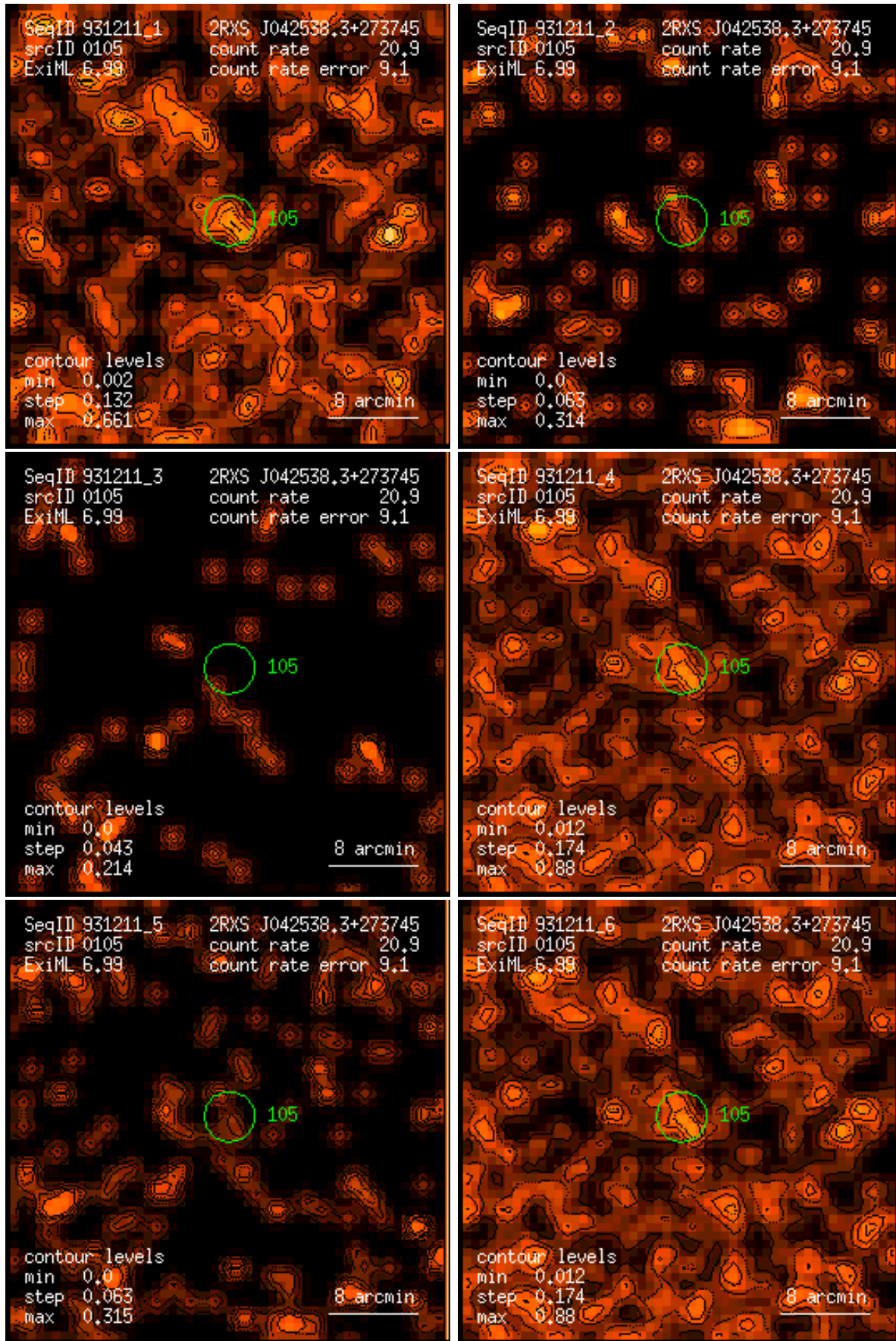
Figure 105: RASS 931211: detection 0105: band rate images, Gaussian filter: (1) PSPPC channels 11 – 41, (2) 52 – 90, (3) 91 – 201, (4) 11 – 235, (5) 52 – 201, (6) 11 – 201. Broad band rates in counts/ks. Band rate contour levels in counts/ks/arcmin 2 .
