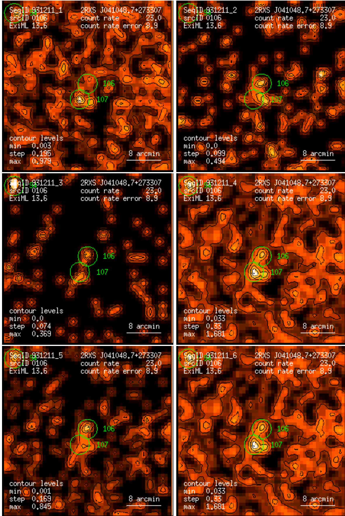
Figure 106: RASS 931211: detection 0106: band rate images, Gaussian filter: (1) PSPC channels 11 – 41, (2) 52 – 90, (3) 91 – 201, (4) 11 – 235, (5) 52 – 201, (6) 11 – 201. Broad band rates in counts/ks. Band rate contour levels in counts/ks/arcmin 2 .
