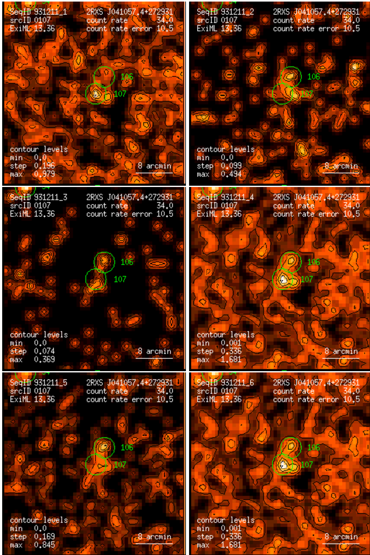
Figure 107: RASS 931211: detection 0107: band rate images, Gaussian filter: (1) PSPC channels 11 – 41, (2) 52 – 90, (3) 91 – 201, (4) 11 – 235, (5) 52 – 201, (6) 11 – 201. Broad band rates in counts/ks. Band rate contour levels in counts/ks/arcmin 2 .
