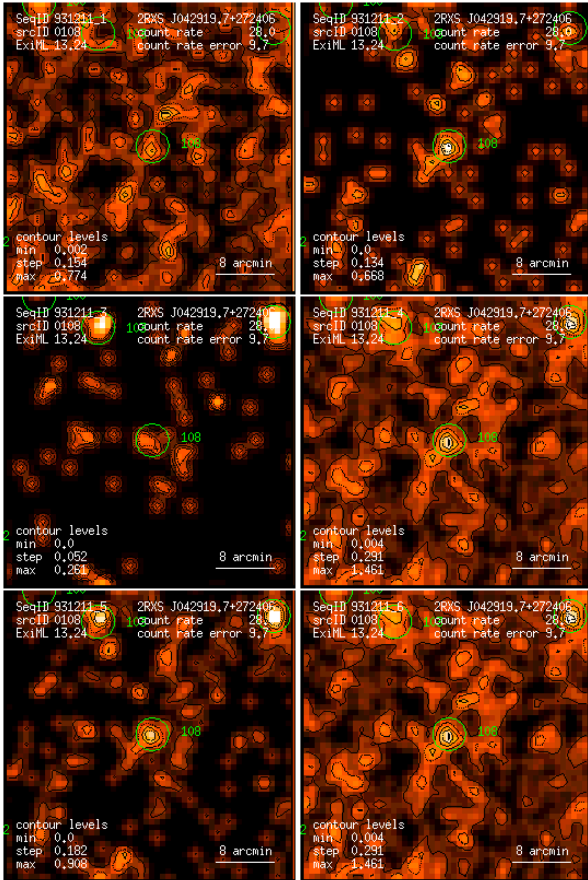
Figure 108: RASS 931211: detection 0108: band rate images, Gaussian filter: (1) PSPC channels 11 – 41, (2) 52 – 90, (3) 91 – 201, (4) 11 – 235, (5) 52 – 201, (6) 11 – 201. Broad band rates in counts/ks. Band rate contour levels in counts/ks/arcmin 2 .
