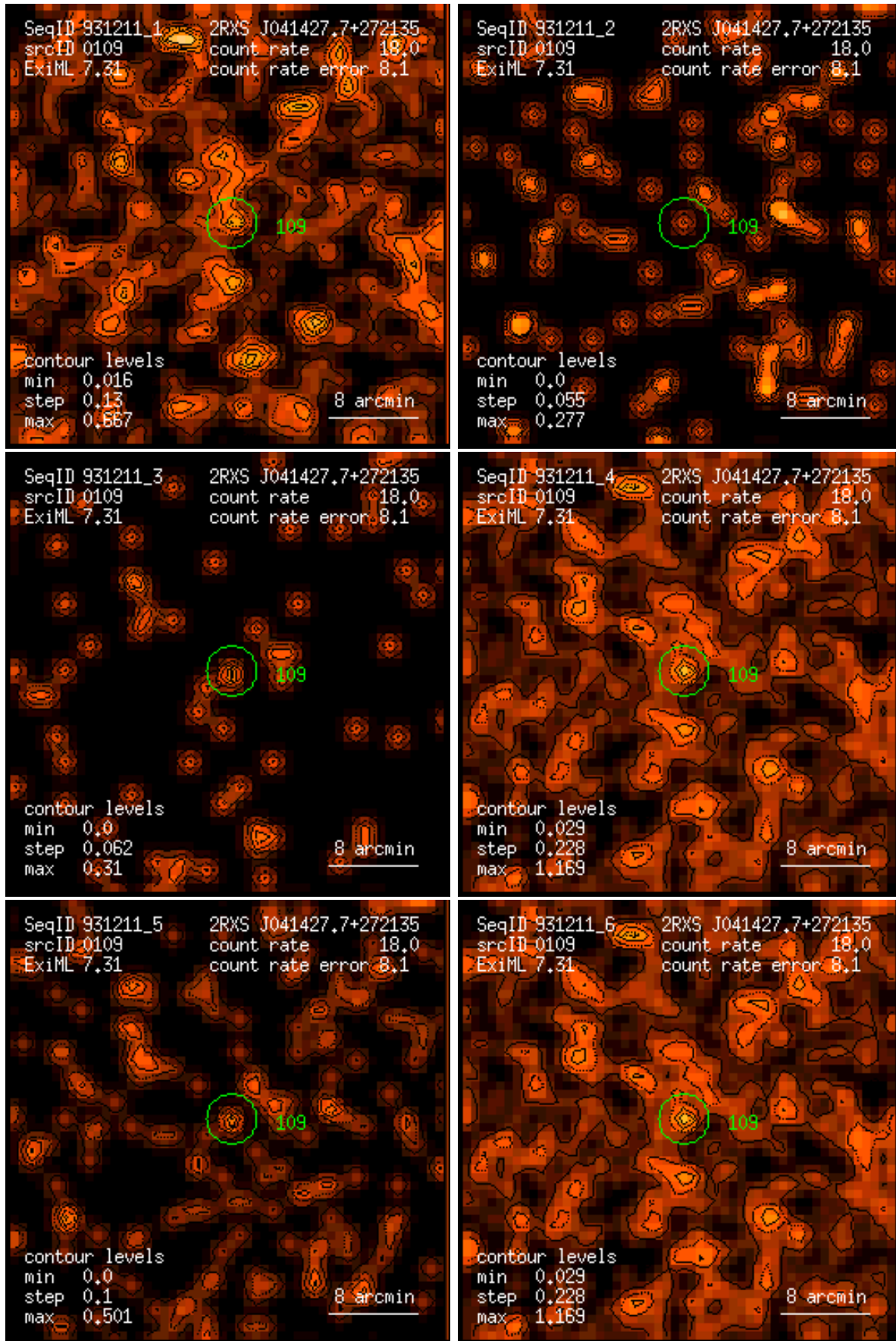
Figure 109: RASS 931211: detection 0109: band rate images, Gaussian filter: (1) PSPC channels 11 – 41, (2) 52 – 90, (3) 91 – 201, (4) 11 – 235, (5) 52 – 201, (6) 11 – 201. Broad band rates in counts/ks. Band rate contour levels in counts/ks/arcmin 2 .
