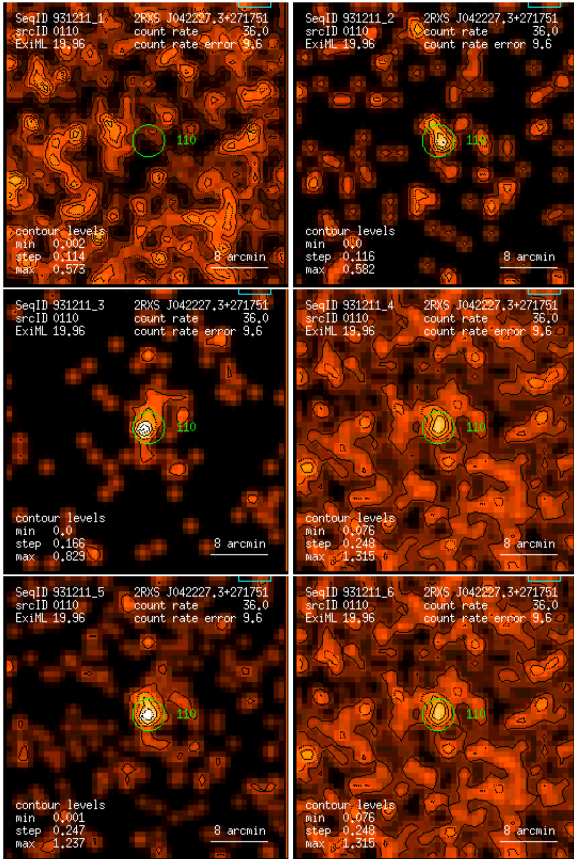
Figure 110: RASS 931211: detection 0110: band rate images, Gaussian filter: (1) PSPC channels 11 – 41, (2) 52 – 90, (3) 91 – 201, (4) 11 – 235, (5) 52 – 201, (6) 11 – 201. Broad band rates in counts/ks. Band rate contour levels in counts/ks/arcmin 2 .
