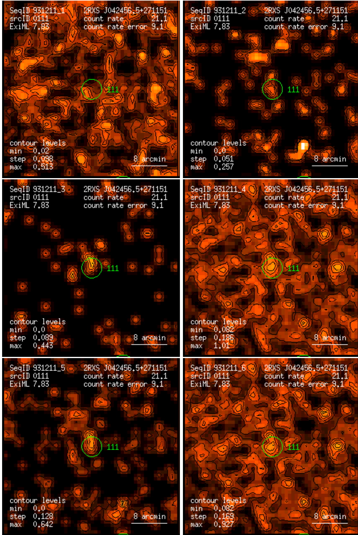
Figure 111: RASS 931211: detection 0111: band rate images, Gaussian filter: (1) PSPC channels 11 – 41, (2) 52 – 90, (3) 91 – 201, (4) 11 – 235, (5) 52 – 201, (6) 11 – 201. Broad band rates in counts/ks. Band rate contour levels in counts/ks/arcmin 2 .
